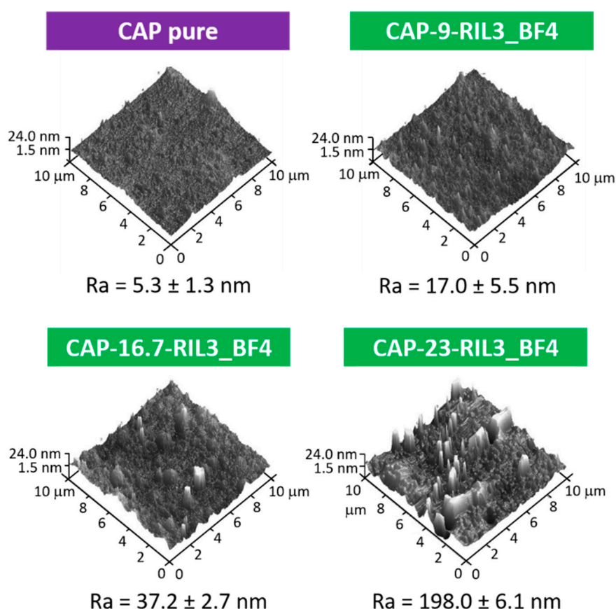
Figure S1. AFM analysis (3D profile) of pristine CAP pure and CAP-RIL3_BF4 films.
