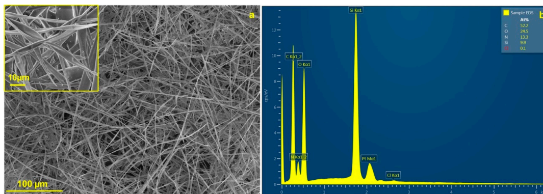
Figure 2. SEM image of the prepared hybrid fibres with an inset showing the helical structure of the parts of the fibres a); Energy Dispersive X-Ray Spectroscopy (EDS) spectra of the hybrid fibres b).
