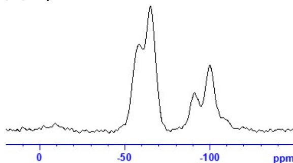
Figure 4. ^{29}\text{Si} CP/MAS NMR spectra of the hybrid DACHsilane fibres.
