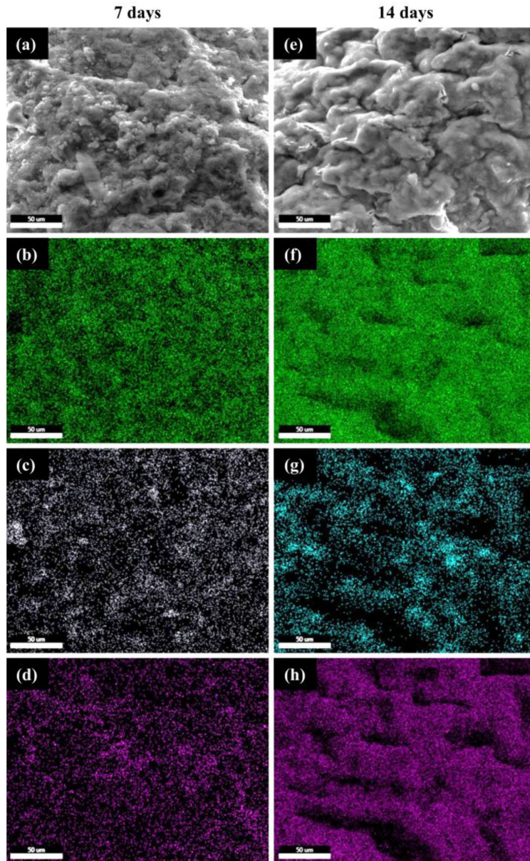
Figure 6. SEM/EDX micrographs with the elemental mapping for CS-FG3 scaffolds after 7 days and 14 days of immersion in SBF (scalebar 50 µm): (a), (e) SEM micrographs representative for the investigated areas, (b), (f) Ca mapping, (c), (g) Si mapping, and (d), (h) P mapping.
