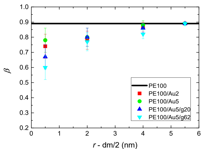
Figure 9. The stretch exponent \beta , as extracted from the fit with KWW functions, of the end-to-end vector ACF, C_{end-end}(t) , as a function of distance from the center of the Au NP, r , minus the half diameter of the NP for all systems with PE matrices consisting of 100 mers per chain. Black lines represent \beta values of bulk PE chains.
