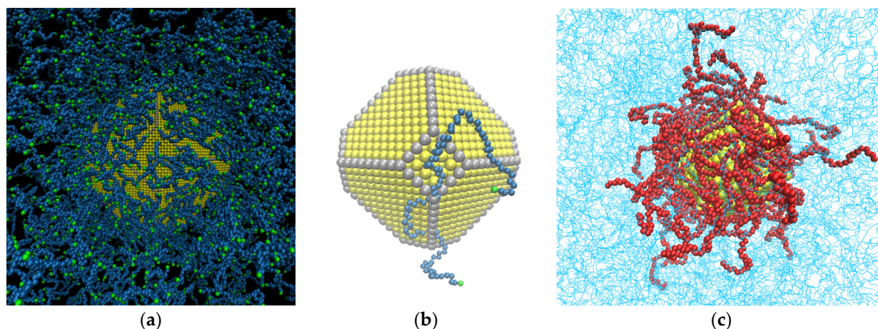
Figure 1. Snapshots from the model systems: (a) The PE22/Au5 hybrid system. In yellow is the Au, in blue are the CH 2 monomers and in green are the CH 3 monomers. (b) Au NP, of d = 5.02 nm (in yellow are the Au atoms and in grey the edge Au atoms), and a PE 100 mer chain. (c) The PE100/Au5/g62 hybrid system. In blue are the free CH 2 and the free CH 3 monomers. In red are the grafted CH 2 and CH 3 monomers.
