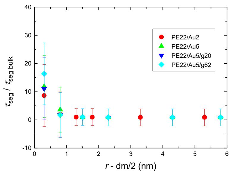
Figure A9. Segmental relaxation times of PE chains, scaled with the value of bulk chains, \tau_{seg}/\tau_{seg bulk} , as a function of distance from the center of the Au NP, r , minus the half diameter of the NP, for all systems with PE matrices consisting of 22 mers per chain.
