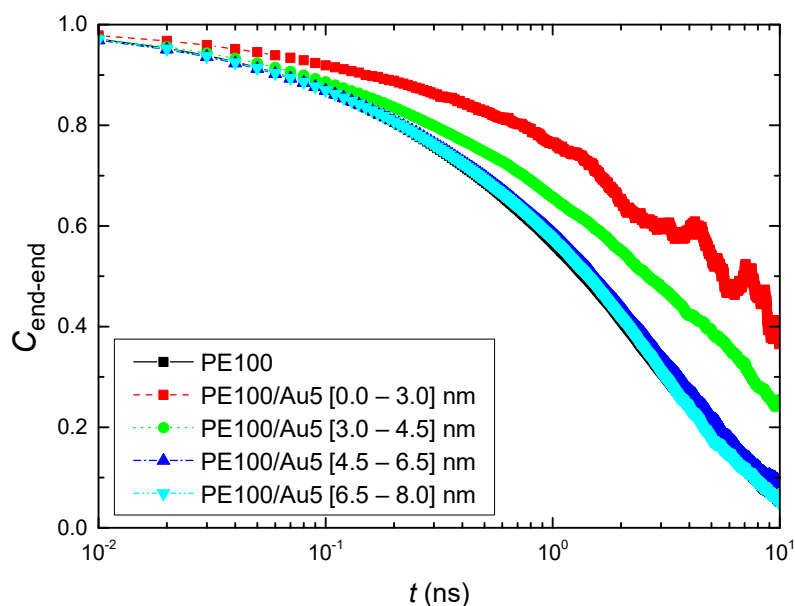
Figure 7. The reorientation time autocorrelation function (ACF) C_{\text{end-end}}(t) as a function of time for the end-to-end vector of polyethylene for PE100/Au5 system. PE chains are analyzed across various shells from the Au NP.
