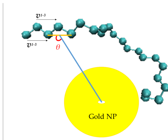
Figure A3. The definition of the \theta angle for the calculation of the second rank bond order parameter S_{1-3} of polyethylene chains for v^{1-3} vector. In blue is the PE and in yellow is the Au NP. The orange line connects two non-consecutive carbon atoms and the blue line connects the center of the gold NP with the midpoint of the orange line. In red is the \theta angle.
