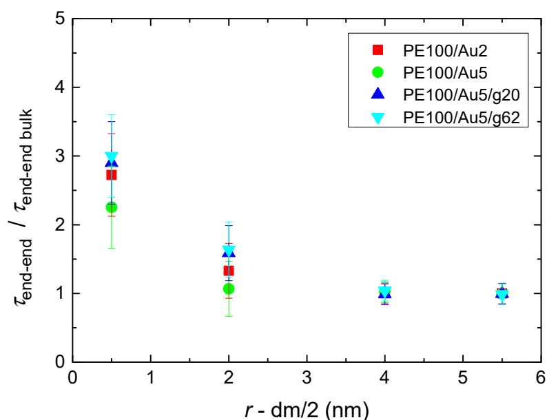
Figure 8. Relaxation time of the end-to-end vector of PE chains, scaled with the value of bulk chains, \tau_{end-end}/\tau_{end-end bulk} , as a function of distance from the center of the Au NP, r , minus the half diameter of the NP, for all systems with PE matrices consisting of 100 mers per chain.
