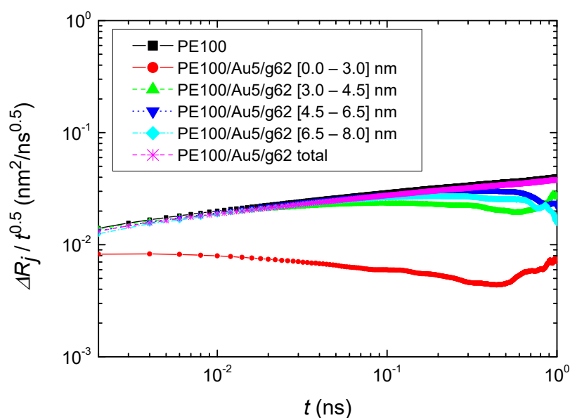
Figure 10. Segmental MSD of PE chains along r (distance from the center of the gold NP), \Delta R_j , scaled with t^{0.5} . Data for the PE100/Au5/g62 system, for various spherical shells, and the total MSD of the PE100 and PE100/Au5/g62 systems are shown.
