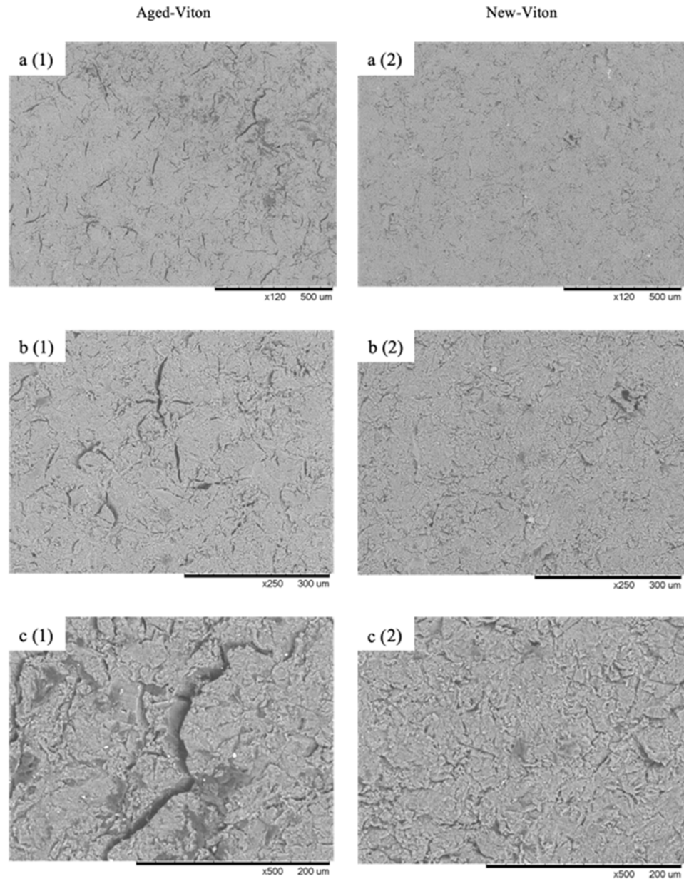
Figure 6. SEM micrographs of the new and aged Viton sample. (a) \times 120 , (b) \times 250 , (c) \times 500 magnification.
