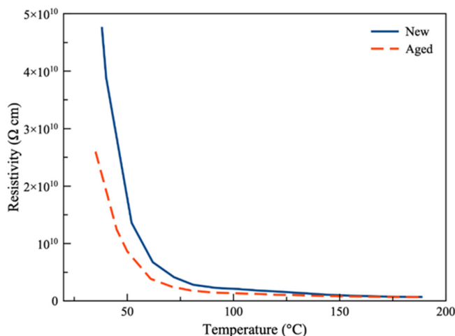
Figure 4. Volume resistivity of Viton specimen at various temperatures ranging from 35 to 190 °C at 500 V (less than 2% error).
