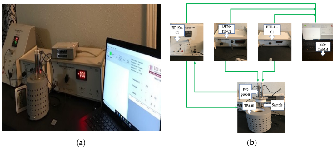
Figure 1. Resistivity measurement setup 1 (TPX-200 C). (a) Overall setup, (b) block diagram of connections.
