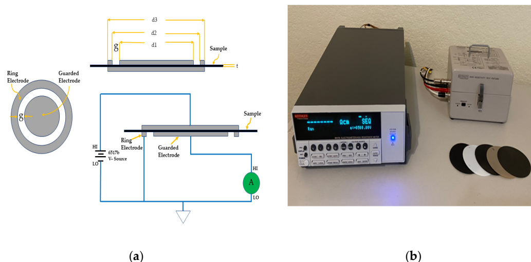
Figure 2. (a) Schematic of a typical electrometer resistivity test; (b) resistivity measurement setup 2 (Keithley 6517b + 8009).
