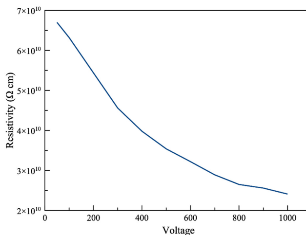
Figure 5. Volume resistivity of Viton specimen under various voltages (less than 1% error).
