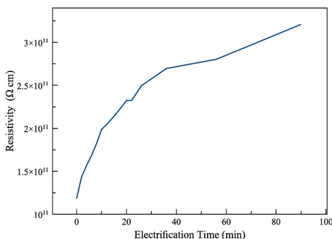
Figure 3. Volume resistivity with respect to time of a Viton sample under constant 500 V DC (less than 1% error).
