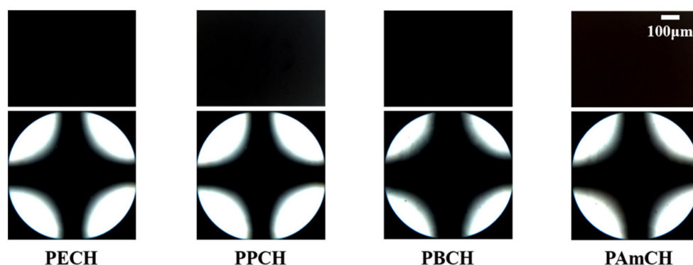
Figure 4. Orthoscopic (top) and conoscopic (bottom) polarized optical microscopy (POM) images of the LC cells fabricated with PECH, PPCH, PBCH, and PAmCH films.
