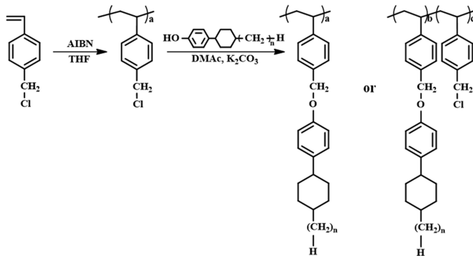
Figure 1. Synthetic route to 4-( trans -4-ethylcyclohexyl)phenoxy-methyl (PECH# and PECH, n = 2 ), 4-( trans -4-propylcyclohexyl)phenoxy-methyl (PPCH, n = 3 ), 4-( trans -4-butylcyclohexyl)phenoxy-methyl (PBCH, n = 4 ), and 4-( trans -4-amylcyclohexyl)phenoxy-methyl-substituted polystyrene (PAmCH, n = 5 ), where # represents the molar fraction of 4-( trans -4-ethylcyclohexyl)phenol containing monomeric units in the polymer.
