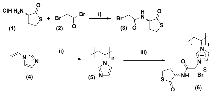
Scheme 1. Synthesis of PIL 6 . (i) \text{K}_2\text{CO}_3 , \text{H}_2\text{O}/\text{CH}_2\text{Cl}_2 0\text{ }^\circ\text{C} , then rt. (ii) AIBN, 100\text{ }^\circ\text{C} , 24 h DMF. (iii) DMF, 80\text{ }^\circ\text{C} , 24 h.
