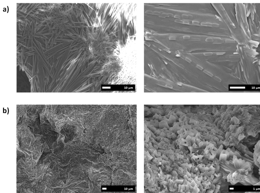
Figure 6. Sem pictures for the polymeric mats (a) Mat 7 (scale bars correspond to 10 µm) (b) Mat 8 (scale bars correspond to left: 10 µm, right: 1 µm).
