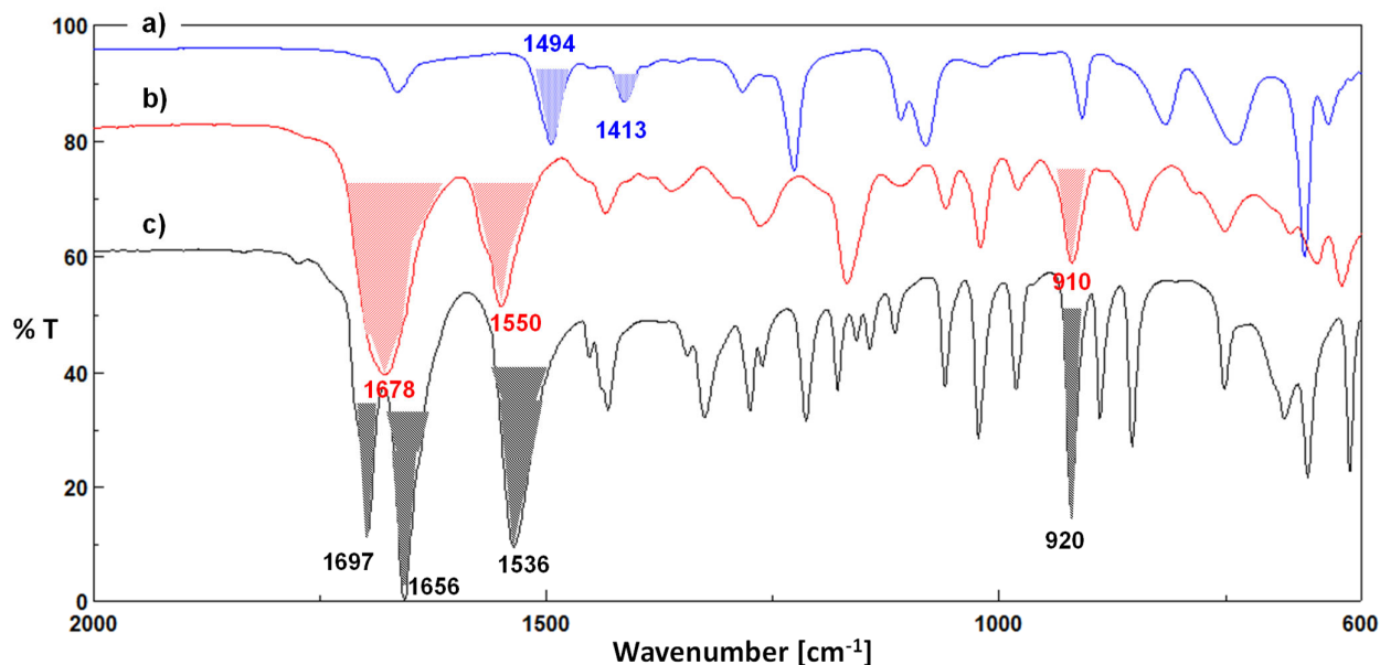
Figure 2. Synthesis of the polymer 6 monitored by ATR-FTIR. (a) Polymer 5 , (b) Polymer TS-PIL 6 and (c) alkylating agent containing amino-thiolactone units ( 3 ).
