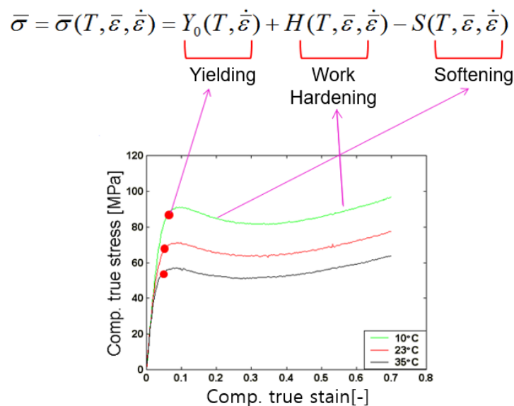
Figure 1. Stress-strain relation of poly methyl methacrylate (PMMA) in the low temperature region.
