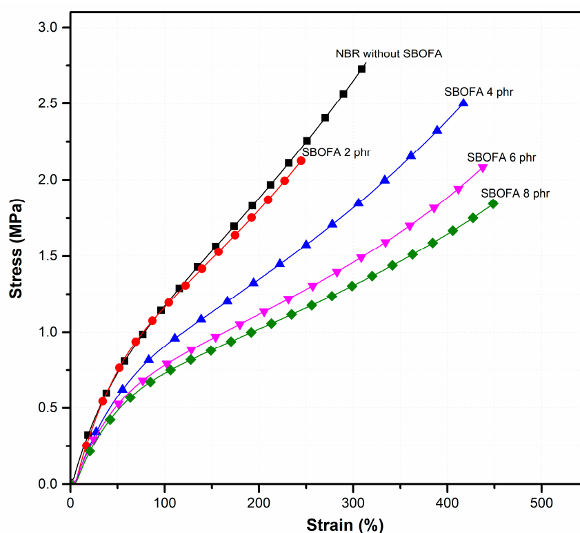
Figure 9. Stress–strain curves of the NBR vulcanizates with varying SBOFA loadings.
