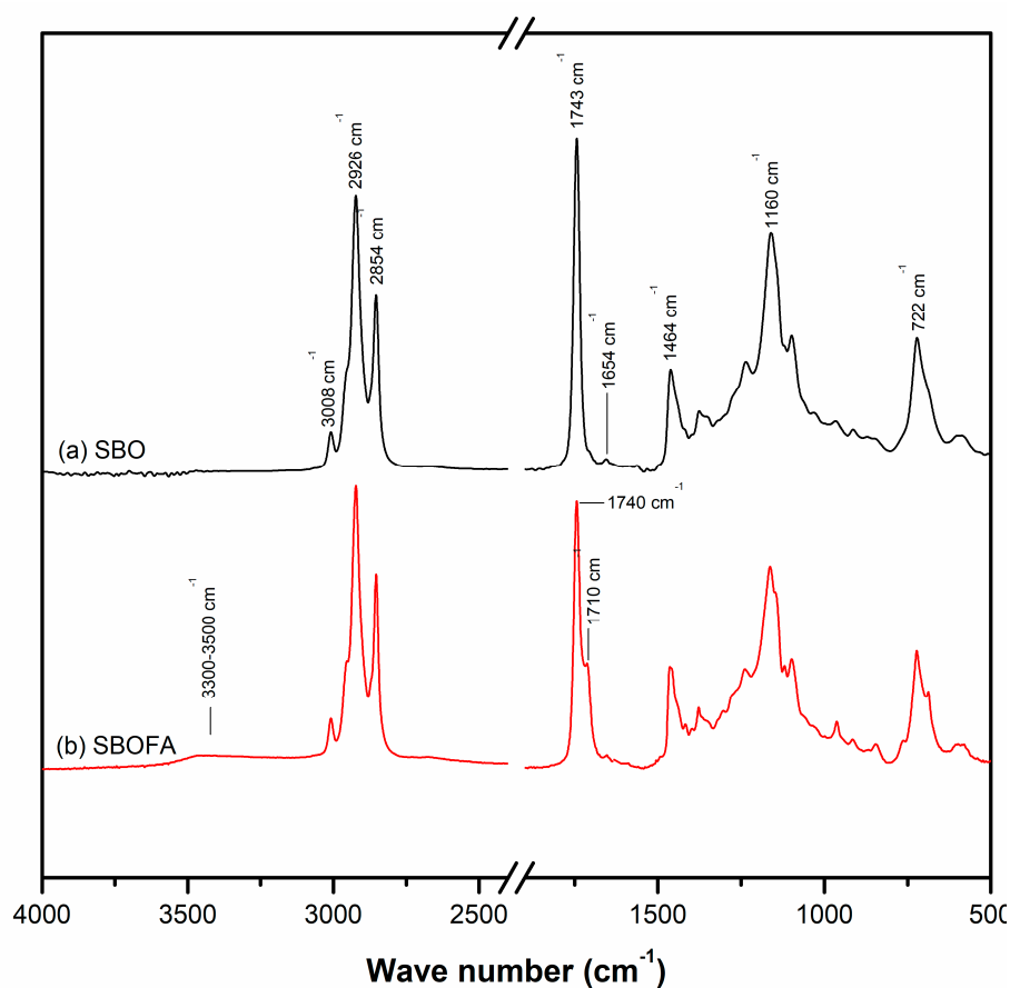
Figure 1. Representative ATR-FTIR spectra of the (a) SBO and (b) SBOFA.
