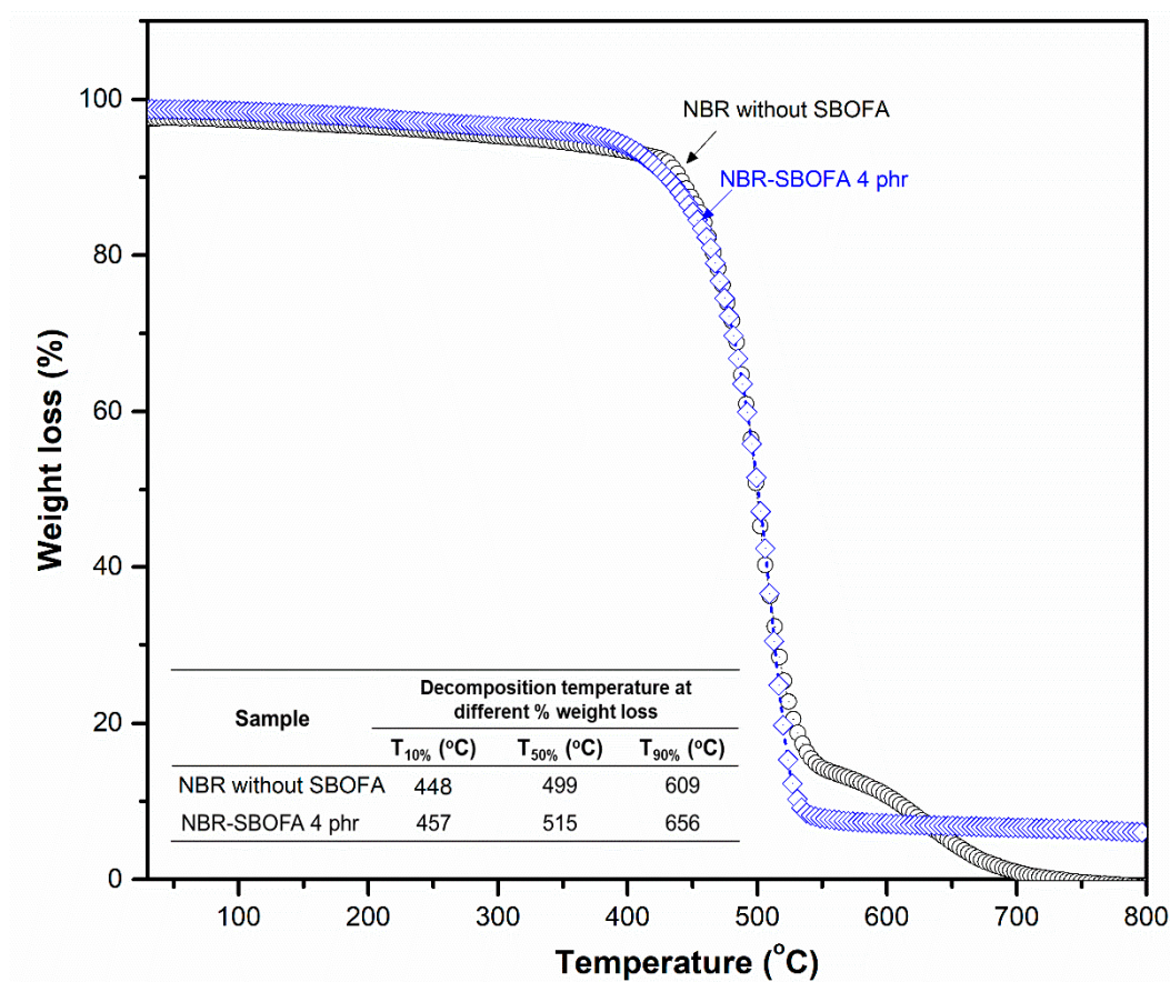
Figure 13. Representative TGA curves of the NBR vulcanizates with SBOFA at 0 and 4 phr.
