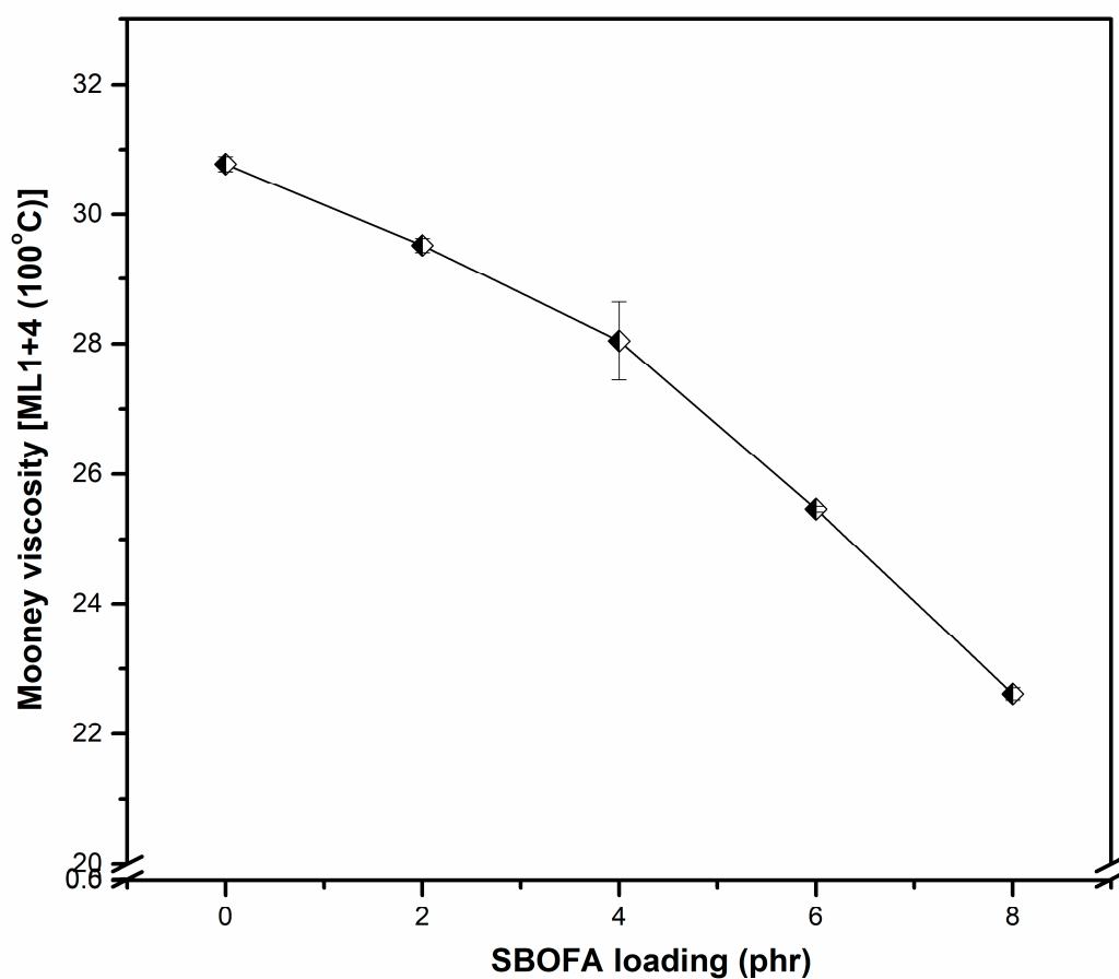
Figure 3. Mooney viscosity of NBR compounds with varying SBOFA loadings. Data are shown as the mean \pm 1SD, derived from three experiments.
