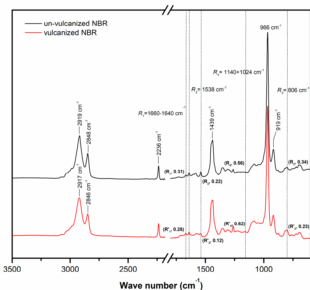
Figure 5. Representative ATR-FTIR spectra of the unvulcanized and peroxide-vulcanized NBR.
