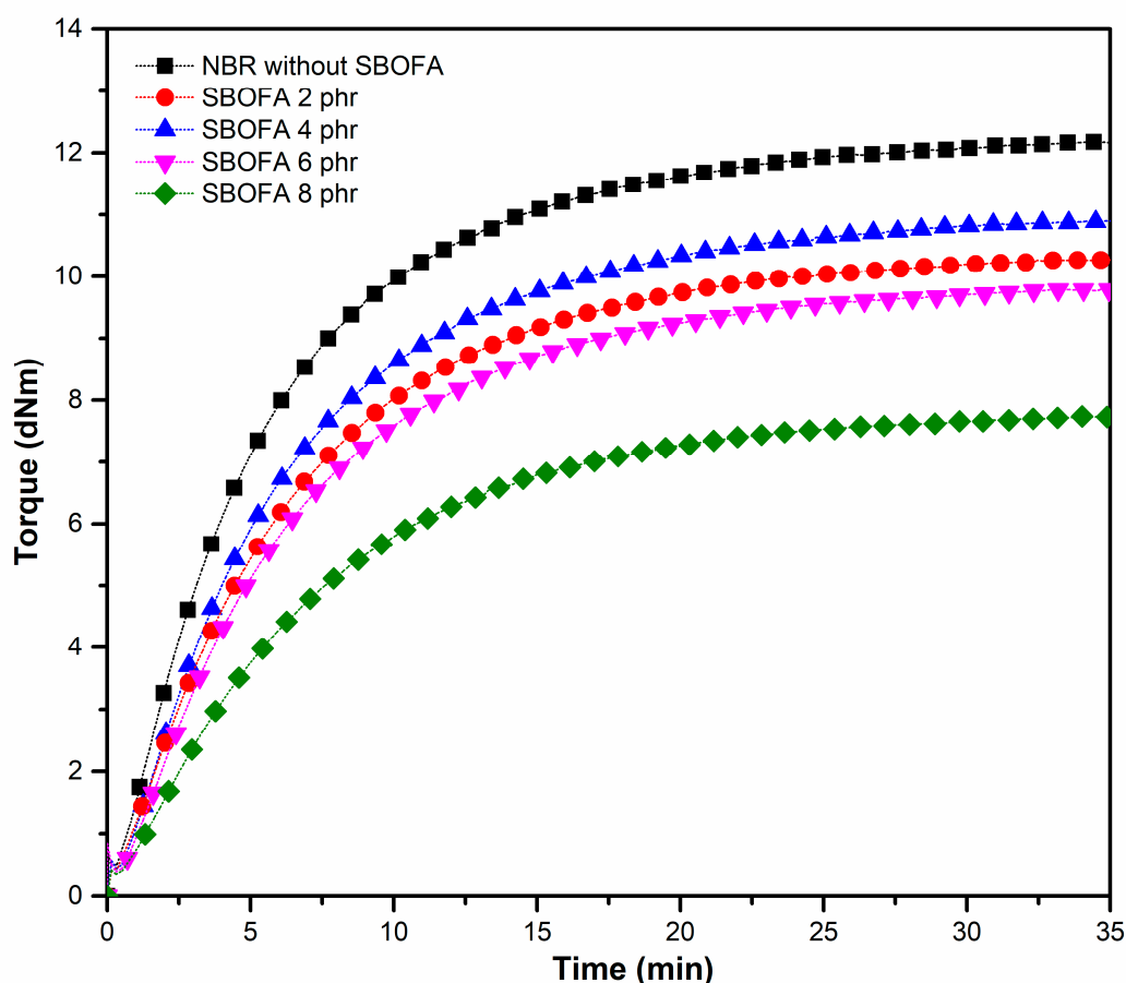
Figure 7. Cure curves of NBR compounds with varying SBOFA loadings.
