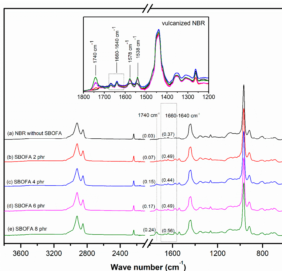
Figure 6. Representative ATR-FTIR spectra of NBR vulcanizates with varying SBOFA loadings.
