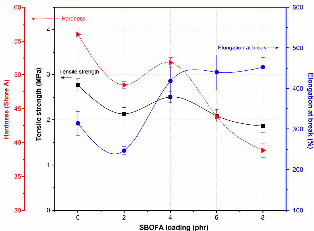
Figure 10. The tensile strength, elongation at break, and hardness of NBR vulcanizates with varying SBOFA loadings. Data of tensile properties and hardness are shown as the mean \pm 1SD, derived from five and three experiments, respectively.
