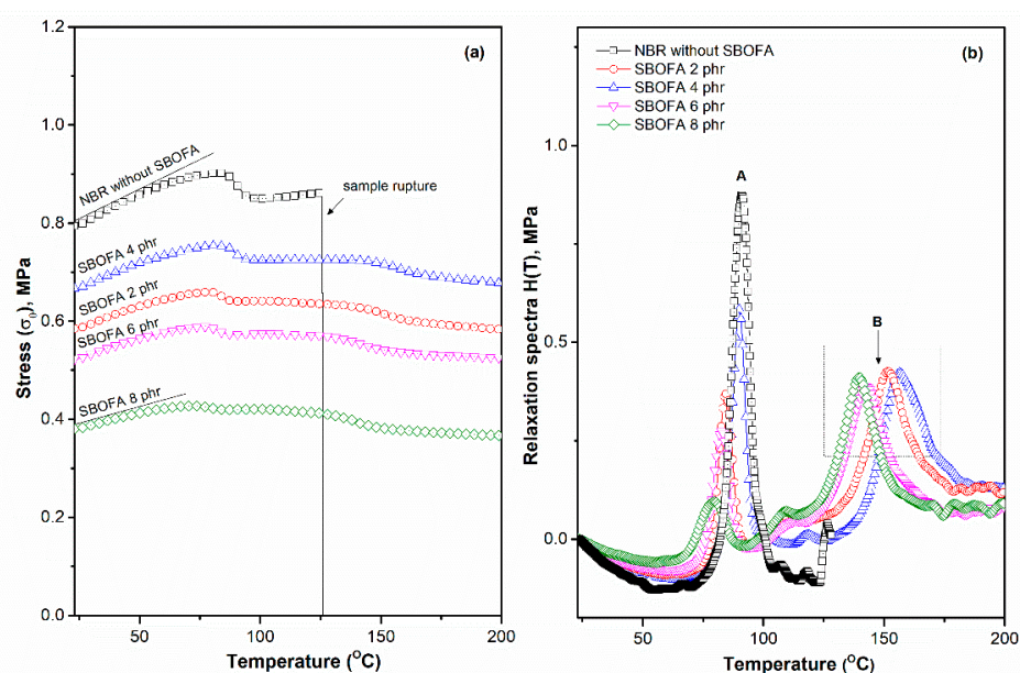
Figure 12. Representative (a) stress ( \sigma_0 ) and (b) relaxation spectra H(T) plots as function of temperature for NBR vulcanizates with varying SBOFA loadings.
