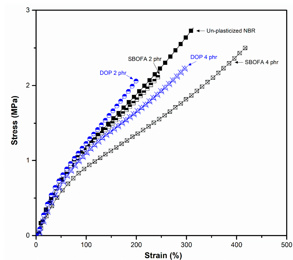
Figure 15. Representative stress–strain curves of unplasticized NBR and NBR vulcanizates with 2 and 4 phr loadings of SBO and DOP.
