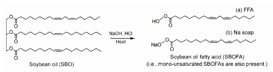
Figure 2. Hydrolysis reaction of SBO and its hydrolyzed products.
