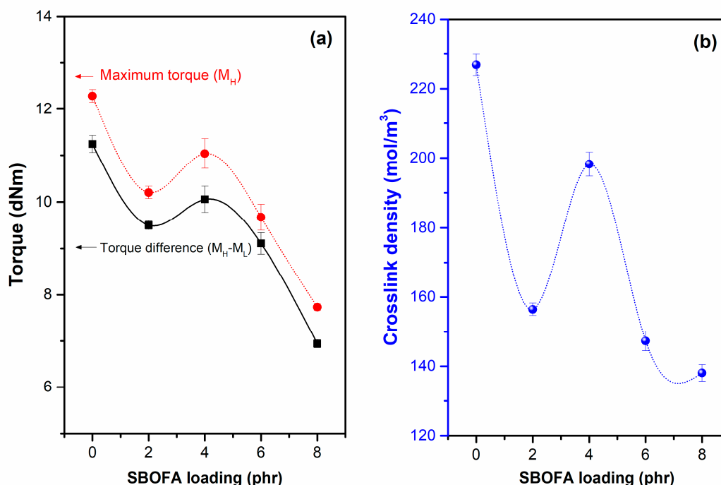
Figure 8. The (a) maximum torque ( M_H ) and torque difference ( M_H - M_L ) and (b) crosslink density of NBR compounds with varying SBOFA loadings. Data are shown as the mean \pm 1 SD, derived from three experiments.
