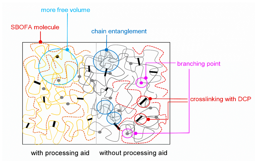
Figure 4. Proposed model for the plasticization with the SBOFA resulting in increasing free volume and chain mobility of the NBR compound.
