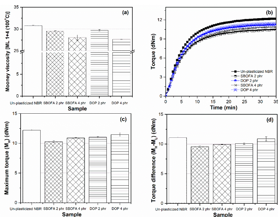
Figure 14. The (a) Mooney viscosity; (b) cure characteristic; (c) maximum torque ( M_H ), and (d) torque difference ( M_H - M_L ) of unplasticized NBR and NBR vulcanizates with 2 and 4 phr of SBO and DOP. Data are shown as the mean \pm 1SD, derived from three experiments.
