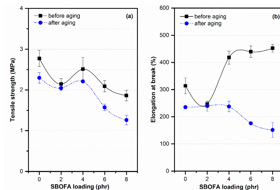
Figure 11. The (a) tensile strength and (b) elongation at break of NBR vulcanizates with varying SBOFA loadings before and after thermal aging at 100°C for 48 h. Data are shown as the mean \pm 1SD, derived from five experiments.
