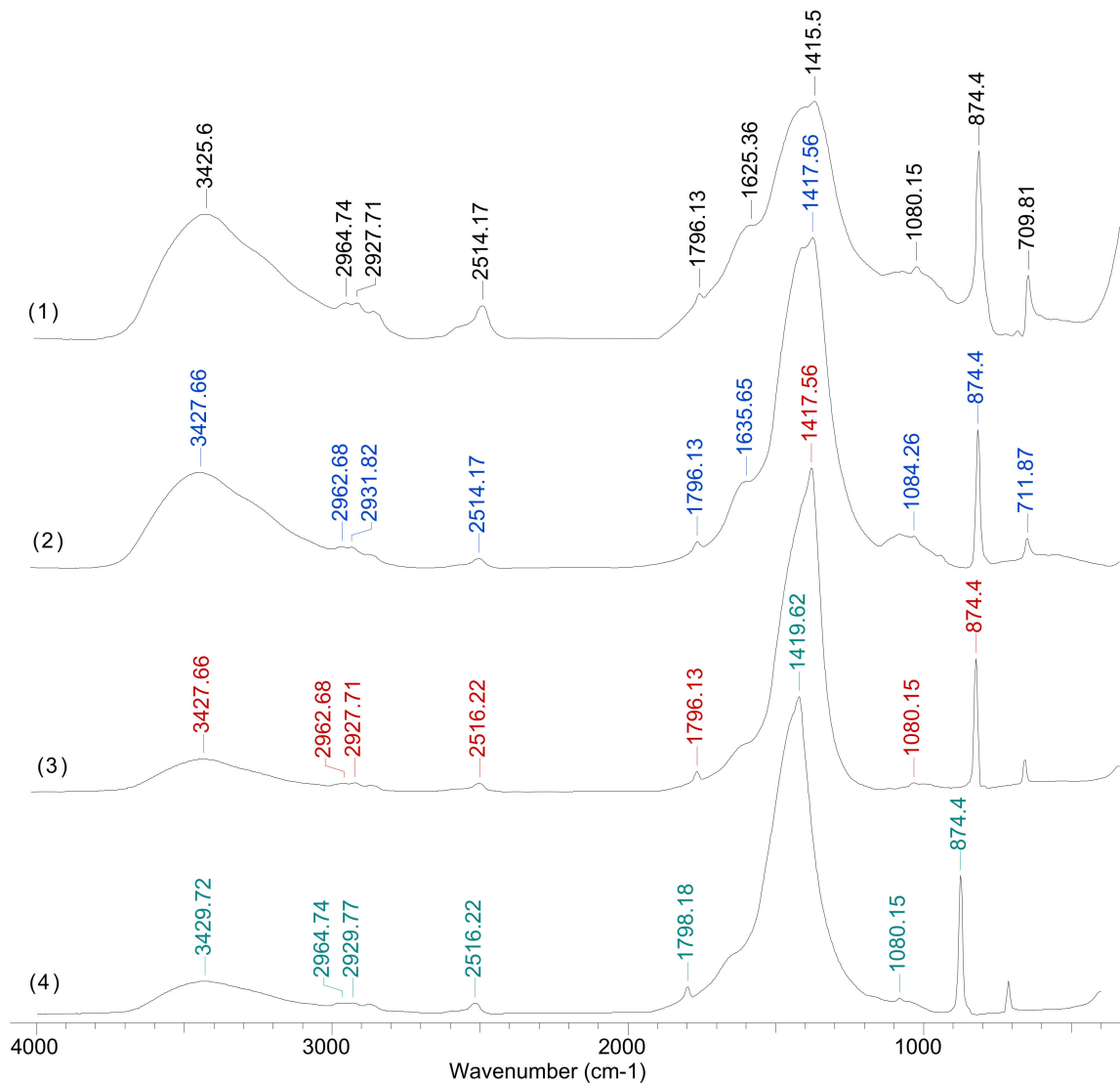
Figure 7. FTIR spectra of Alg-Fe 3 O 4 -MPs before (1) and after biosorption of Cu(II) (2), Co(II) (3) and Zn(II) (4) ions from aqueous media.
