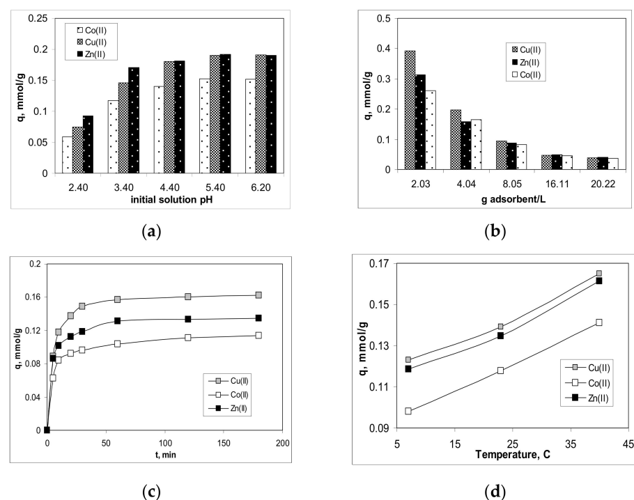
Figure 3. Effect of initial solution pH (a), adsorbent dosage (b), contact time (c) and temperature (d) on biosorption of Cu(II), Co(II) and Zn(II) ions on Alg-Fe 3 O 4 -MPs.
