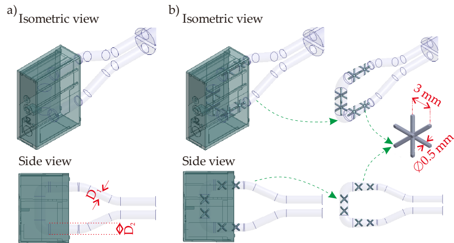
Figure 5. 3D views of the tapered CCCs: (a) tapered and (b) BCC-integrated tapered types.
