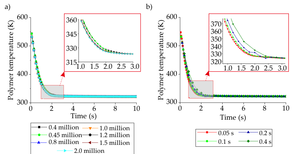
Figure 7. Independence of (a) mesh structure and (b) time-step.
