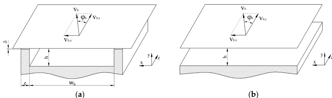
Figure 4. Flat-plate model of the helical screw channel (a). For shallow screw channels with h/w_b < 0.1 , the effect of the screw flights can be ignored (b).
