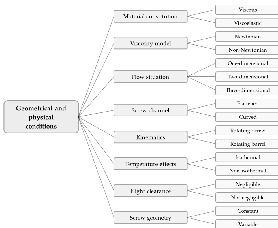
Figure 1. Model categorization A: Classification of melt-conveying models according to the geometrical and physical conditions under consideration.
