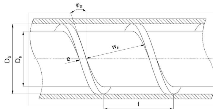
Figure 3. Helical screw channel.
