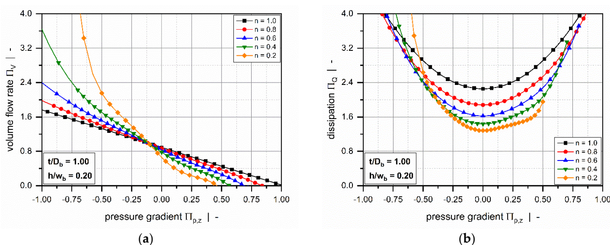
Figure 10. Influence of the power-law index on a fully developed three-dimensional flow of a power-law fluid in a screw channel of finite width under isothermal conditions. The dimensionless volume flow rate \Pi_V as a function of the dimensionless pressure gradient \Pi_{p,z} (a), and the dimensionless dissipation \Pi_Q as a function of the dimensionless pressure gradient \Pi_{p,z} (b).
