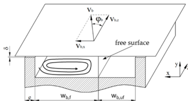
Figure 5. Partially filled screw channel. The widths of the filled and unfilled channel sections are w_{b,f} and w_{b,uf} , respectively.
