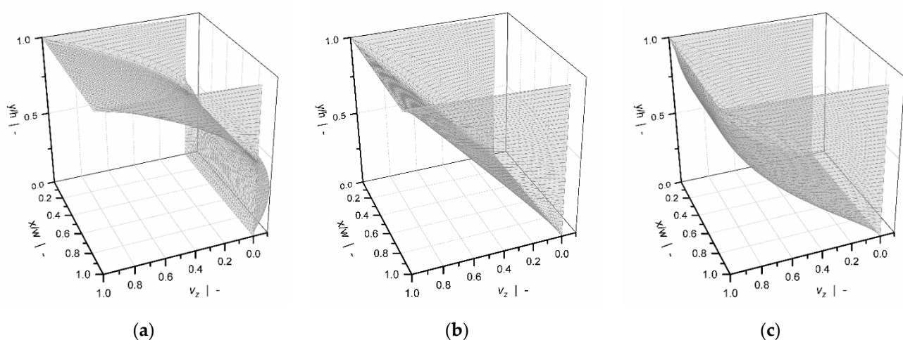
Figure 6. Dimensionless down-channel velocity distribution for a pressure-generating screw section (a), a pressure-neutral screw section (b), and a pressure-consuming screw section (c).
