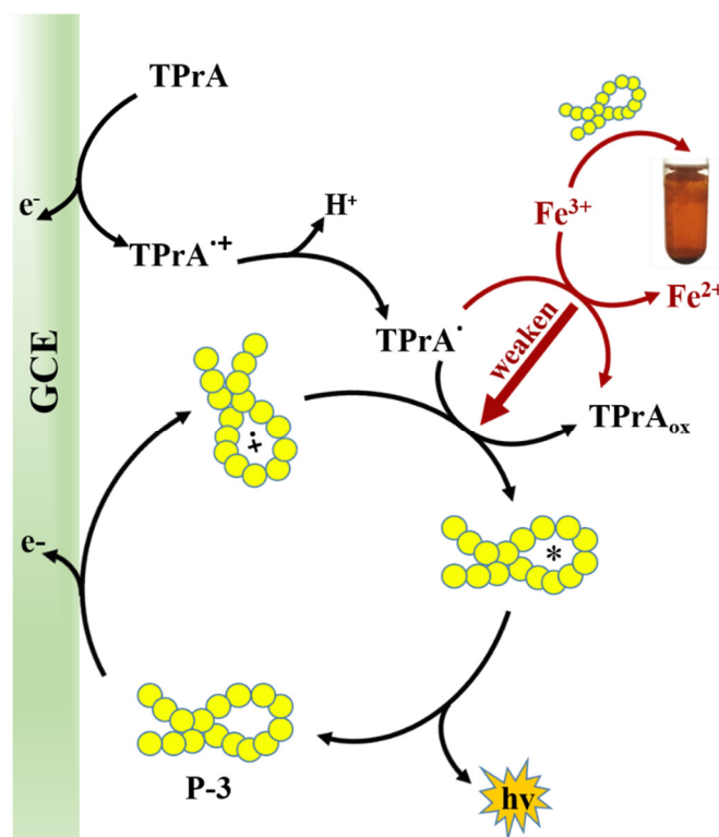
Scheme 2. The possible reaction mechanism: intermolecular electron transfer between P-3 and TPrA and the competition of P-3 and Fe 3+ for TPrA.
