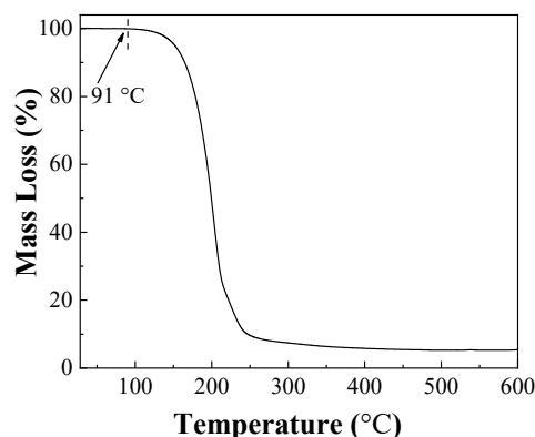
Figure 3. The TG curve of IPBC.
