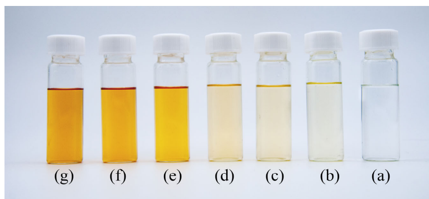
Figure 4. The color changes of IPBC in acetonitrile during thermal degradation at 140 °C for different heating times: (a) 0 min; (b) 10 min; (c) 20 min; (d) 30 min; (e) 40 min; (f) 50 min; and (g) 60 min.
