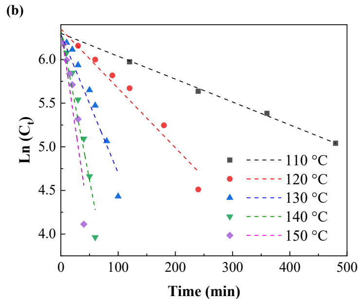
Figure 5. First-order kinetic model for the thermal degradation of IPBC at different heating temperatures: (a) 60–100 °C; (b) 110–150 °C.
