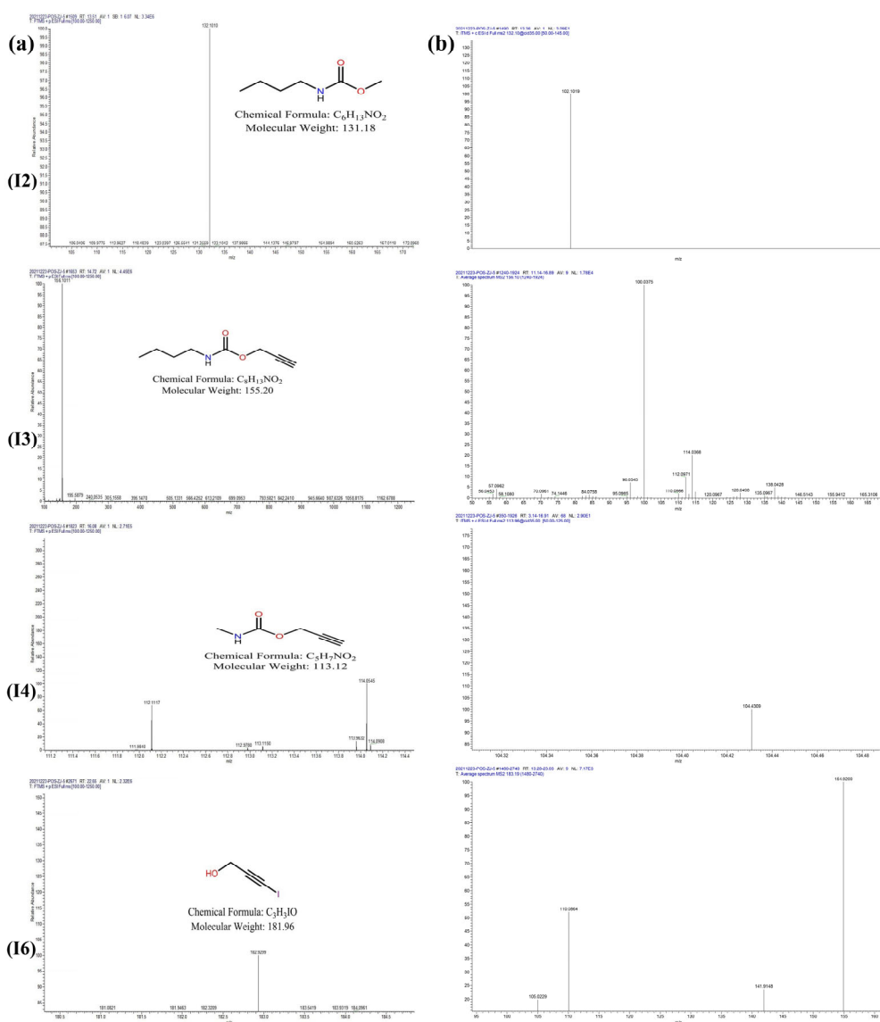
Figure 9. Mass spectrum of degradation products I2, I3, I4, and I6 of IPBC degradation: MS, (a); MS/MS, (b).
