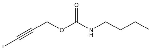
Figure 1. Molecular structure of IPBC.
