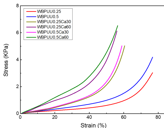
Figure 9. Stress–strain compression curves of WBPUU/CNC and WBPUU/CNC/CaCl 2 scaffolds.
