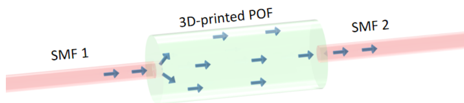
Figure 2. Fibers' mode propagation difference.
