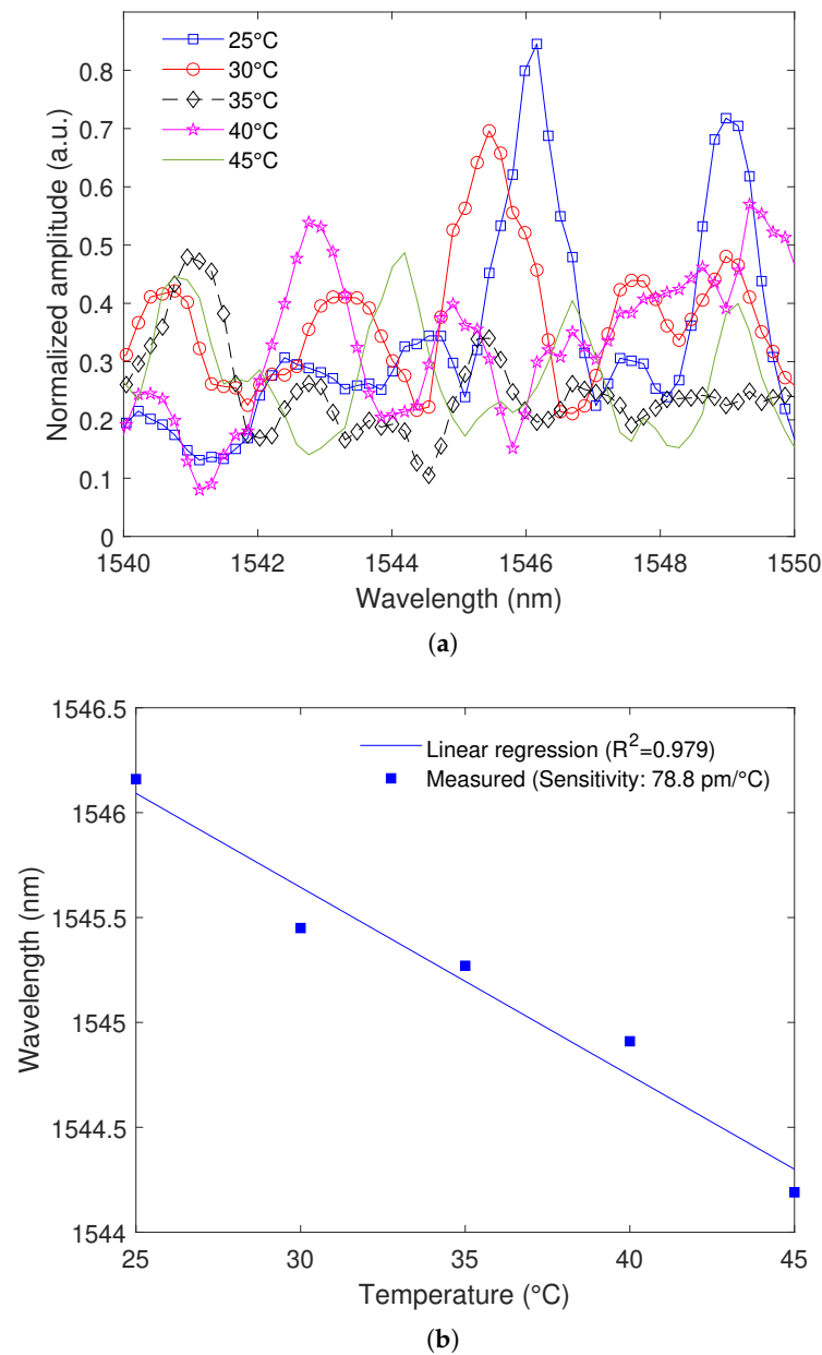
Figure 8. (a) Transmitted spectra as a function of the temperature; (b) Wavelength variation as a function of temperature.
