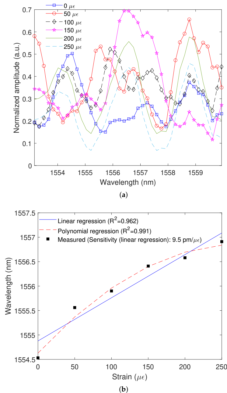
Figure 9. (a) Transmitted spectra as a function of the strain; (b) Wavelength variation as a function of strain for linear and polynomial regressions.
