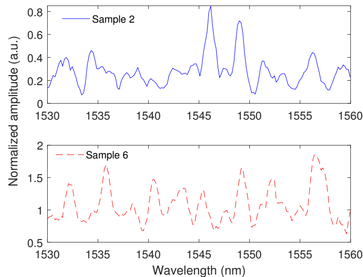
Figure 7. Transmitted spectrum (with normalized optical power) of the proposed SMS interferometer using two samples of the 3D-printed POF.
