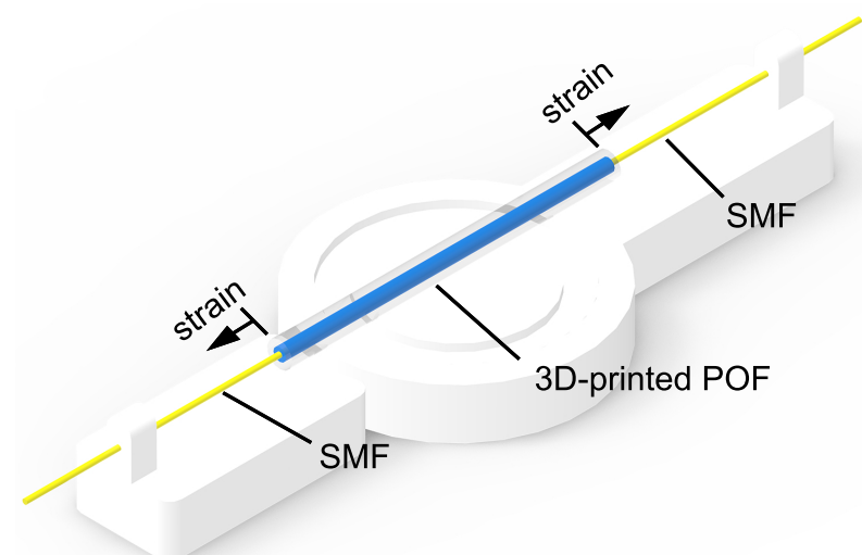
Figure 3. Interferometer strain measure setup.
