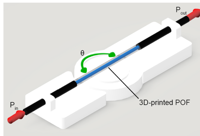
Figure 1. The setup used to measure the change in the intensity of the laser beam with the variation of the angle \theta .
