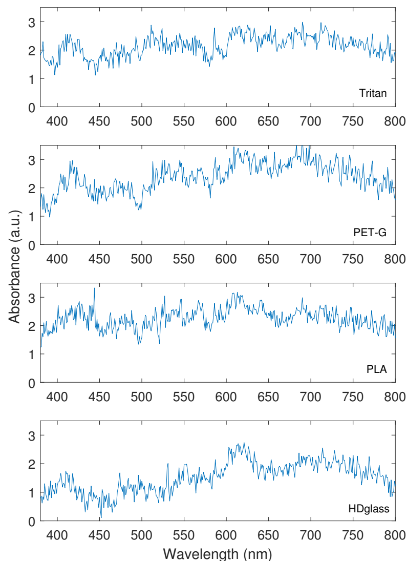
Figure 4. Filament absorbance values measured in the spectrophotometer for the wavelengths where the POFs have the smallest attenuation.
