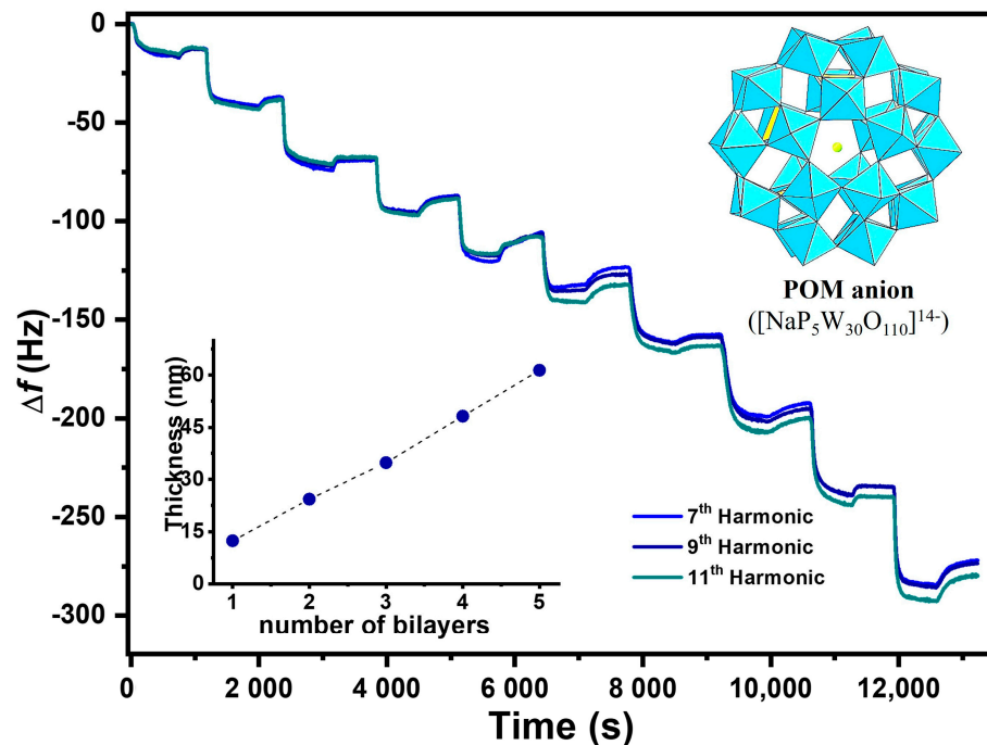
Figure 2. Frequency measurements during LbL assembly were obtained by QCM-D analysis of the (CHT/POM) 5 2D system assembly (from the selected 7th, 9th, and 11th harmonics). Bottom inset: Thickness increases as a function of the bilayer number, obtained using a Voigt viscoelastic model. Top inset: POM anion ( [\text{NaP}_5\text{W}_{30}\text{O}_{110}]^{14-} ) structure representation.
