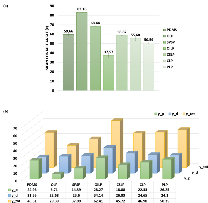
Figure 2. (a) Modifications in surface wettability evaluated by contact angle measurements of PDMS surfaces; (b) Surface free energy components.
