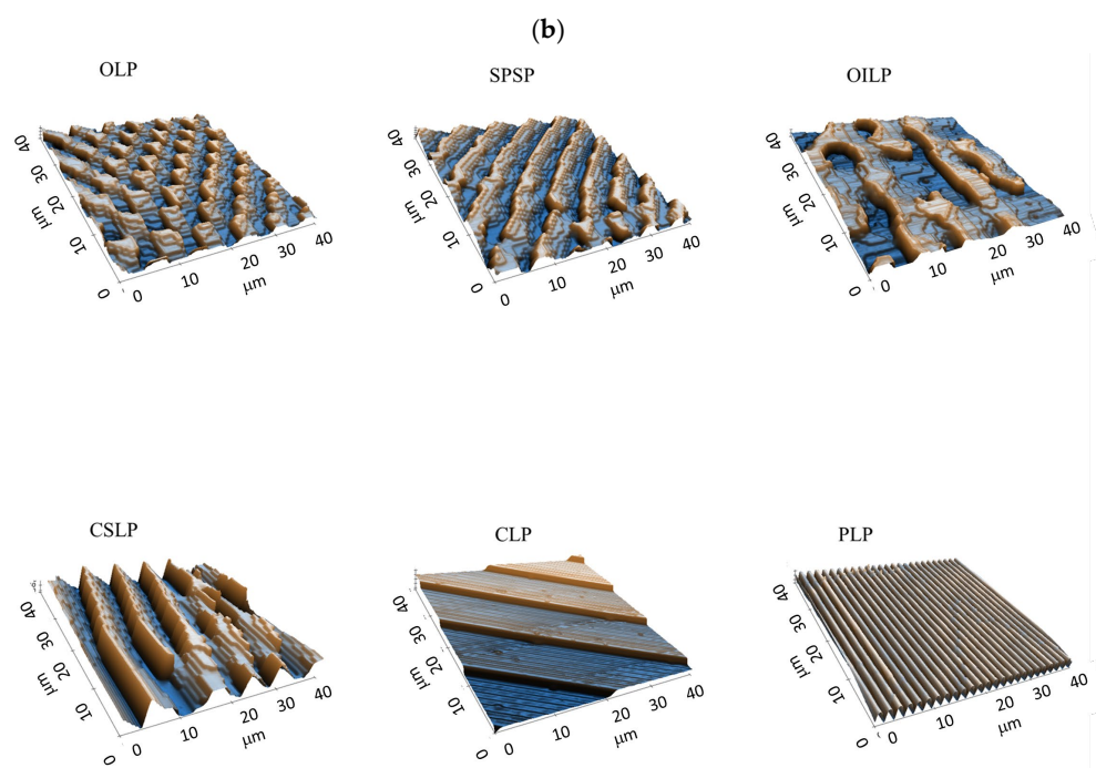
Figure 1. SEM (a) and AFM (b) images of PDMS replicated surfaces depicting step-like structures and the different arrangements on the surface.
