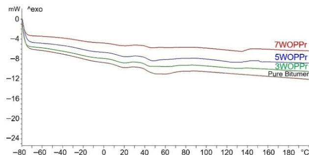
Figure 5. DSC results of the bituminous binders.
