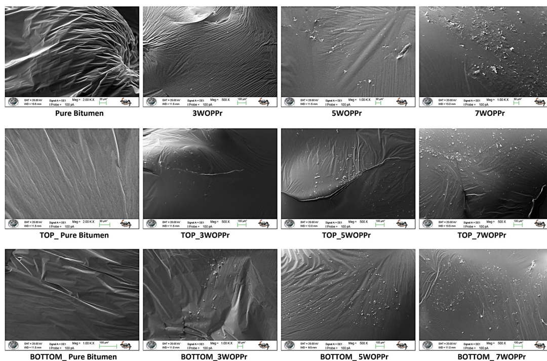
Figure 7. SEM images of bituminous binders.
