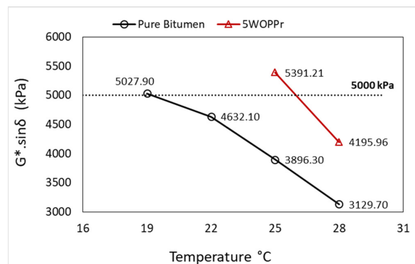
Figure 9. Fatigue parameters of bituminous binders.
