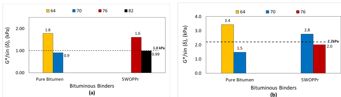
Figure 8. Rutting parameters of bituminous binders: (a) unaged binders, (b) after RTFOT.
