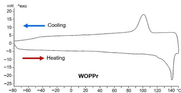
Figure 4. DSC results of the WOPPr.
