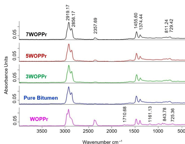
Figure 3. FTIR test results of WOPPr and bituminous binders.
