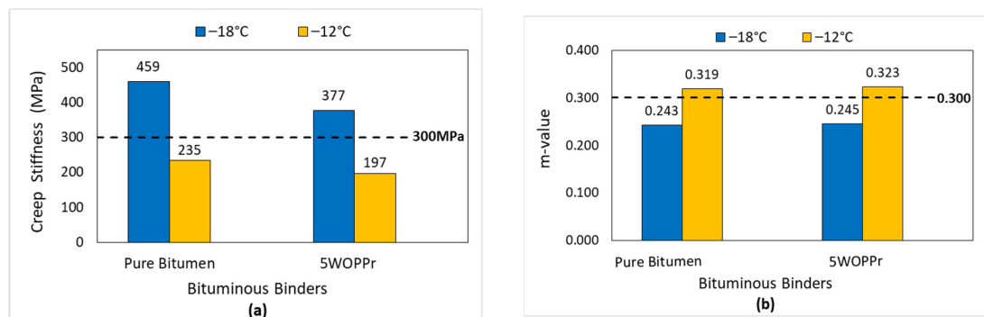
Figure 10. BBR test results of bituminous binders: (a) creep stiffness, (b) m values.
