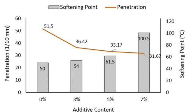
Figure 6. Softening point and penetration values of bituminous binders.
