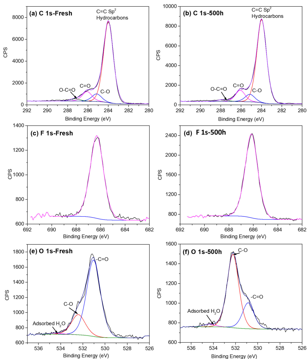
Figure 5. High-resolution XPS spectra of PTQ10:IDIC films deposited on ITO/PEDOT:PSS, recorded in the fresh state (left) and after 500 h of ambient ageing (right). Panels show (a,b) C 1s, (c,d) F 1s, and (e,f) O 1s core-level envelopes. The C 1s spectra are dominated by C–C/C=C, with oxygenated contributions (C–O, O–C=O) reduced after ageing. The F 1s peak increases markedly with time, indicating fluorine surface enrichment, while the O 1s intensity decreases, consistent with oxygen depletion and surface reorganization.
