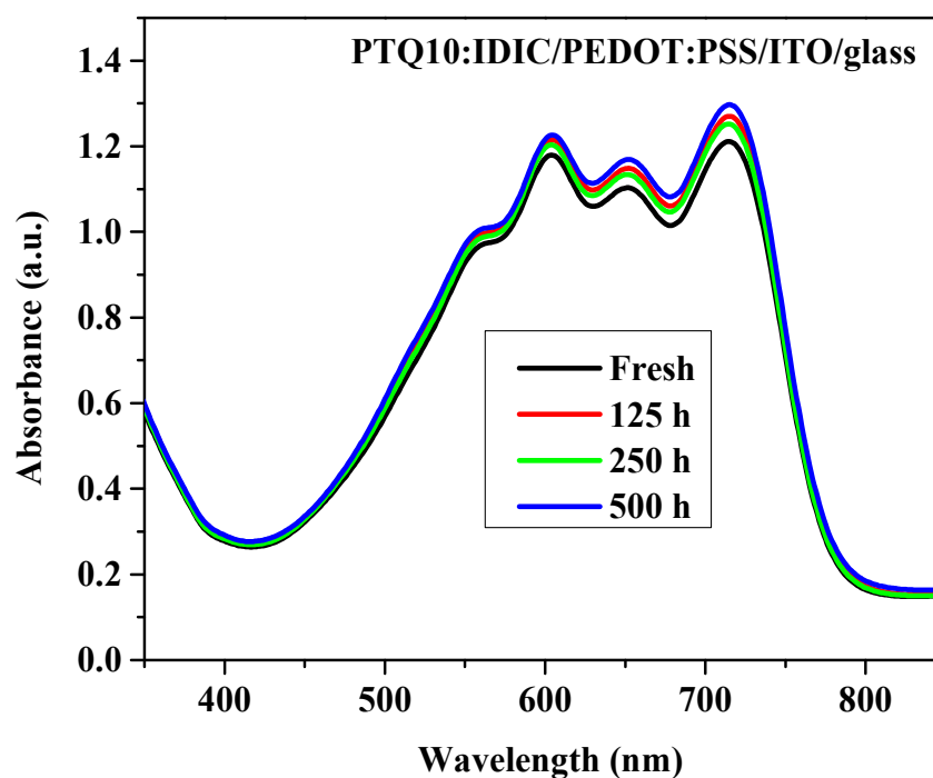
Figure 4. Optical absorption spectra of PTQ10:IDIC films evaluated for up to 500 h of storage in ambient atmosphere.
