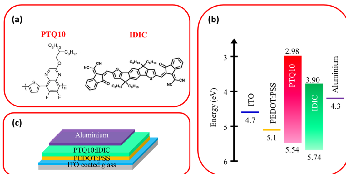
Figure 1. (a) Chemical structure of PTQ10 and IDIC, (b) energy-level diagram of the relevant materials employed in the OSCs. (c) Schematic of the device architecture employed with PTQ10:IDIC photoactive layers.
