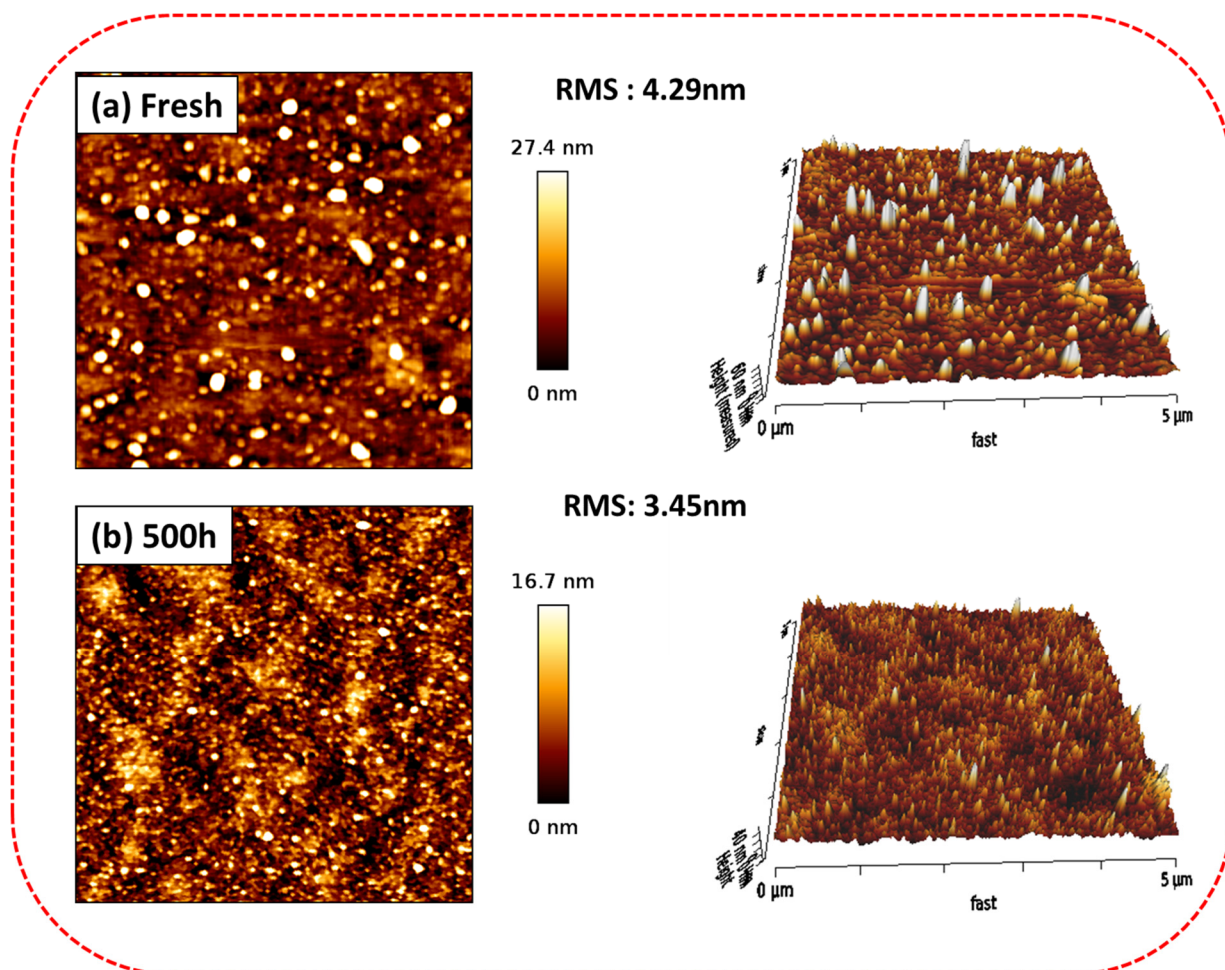
Figure 3. Atomic force microscopy images (2D on the left, 3D on the right) of the PTQ10:IDIC layer after different ageing times. (a) Fresh and (b) aged for 500 h.
