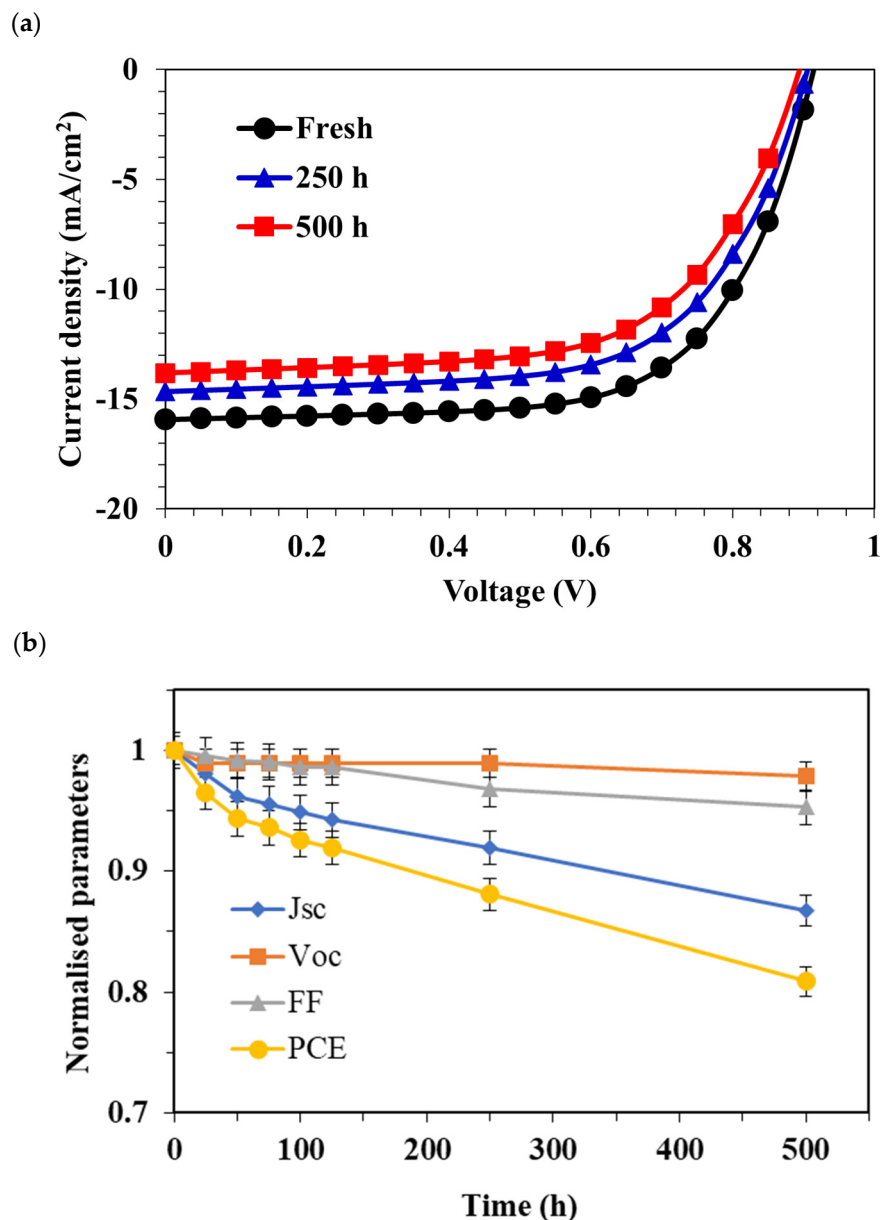
Figure 2. Photovoltaic performance of the OSCs. (a) J - V curves of the OSCs based on PTQ10:IDIC measured after regular interval of time. Device stability of the normal architecture OSCs. (b) Normalized photovoltaic parameters measured up to 500 h of ageing in ambient environment.
