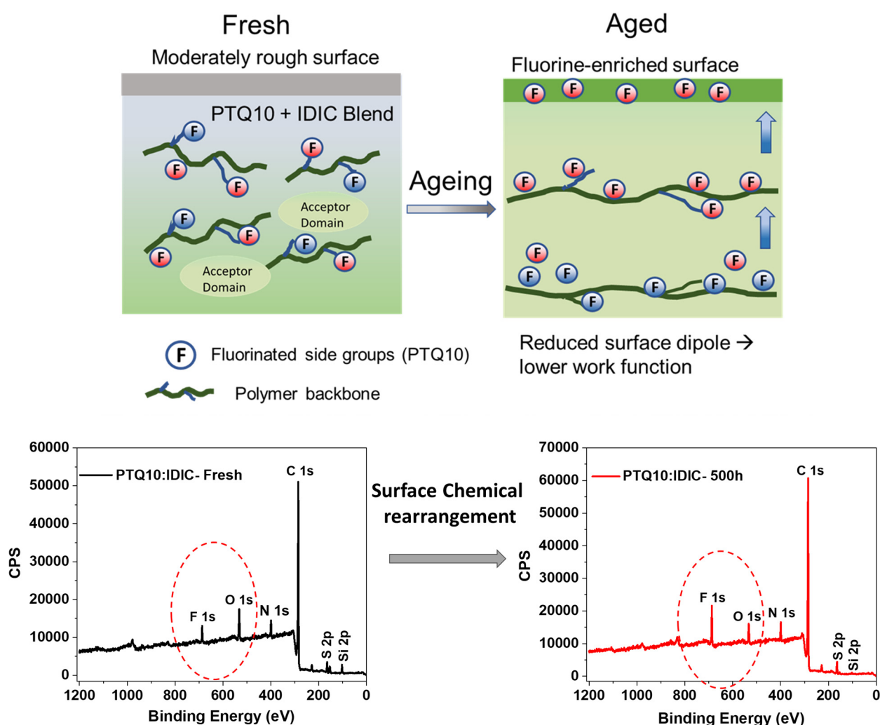
Figure 7. Schematic illustration of interfacial and near-surface evolution in PTQ10:IDIC solar cells during ambient ageing. The fresh film exhibits a moderately rough surface and a mixed near-surface chemical environment, associated with favourable interfacial energetics for charge extraction. Upon ageing, PTQ10 segments containing fluorinated side chains preferentially reorient toward the exposed surface, resulting in fluorine-rich surface termination. Concurrently, oxygen-related surface species become attenuated. These surface reorganizations reduce the effective surface dipole strength and lead to a decrease in the measured work function ( \sim 0.48 eV), while the bulk donor–acceptor morphology and energetics remain largely preserved. The schematic depicts qualitative trends inferred from surface-sensitive measurements and does not imply atomic diffusion or bulk compositional changes.
