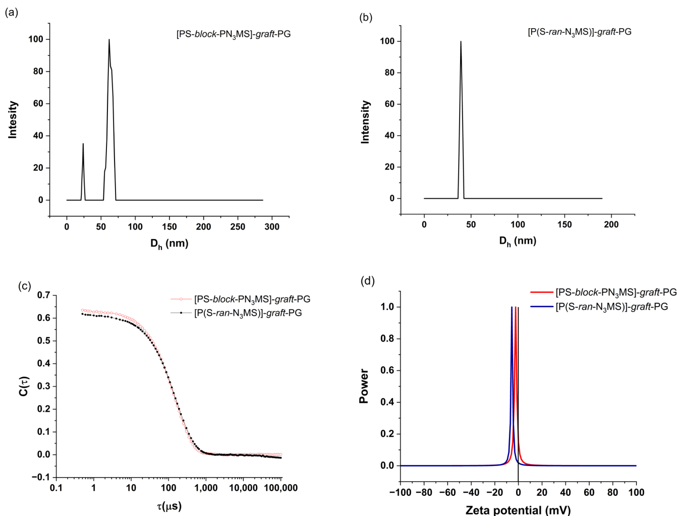
Figure 4. Hydrodynamic diameter ( D_h ) distributions of polymeric micelles prepared by nanoprecipitation: (a) [PS-block-PN 3 MS]-graft-PG and (b) [P(S-ran-N 3 MS)]-graft-PG. (c) Representative intensity correlation functions C(\tau) from DLS measurements. (d) \zeta -potential profiles (red line—[PS-block-PN 3 MS]-graft-PG; blue line—[P(S-ran-N 3 MS)]-graft-PG).
