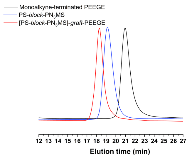
Figure 1. SEC curves of monoalkyne-terminated PEEGE, PS- block -PN 3 MS and resulting [PS- block -PN 3 MS]- graft -PEEGE copolymer.
