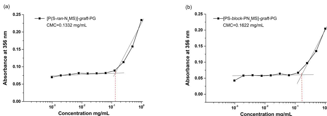
Figure 3. Determination of CMC of the amphiphilic copolymers comprising comb-like and coil-comb chain architecture: (a) [P(S- ran -N 3 MS)]- graft -PG and (b) [PS- block -PN 3 MS]- graft -PG using DPH absorbance at 356 nm in aqueous media at 37 °C.
