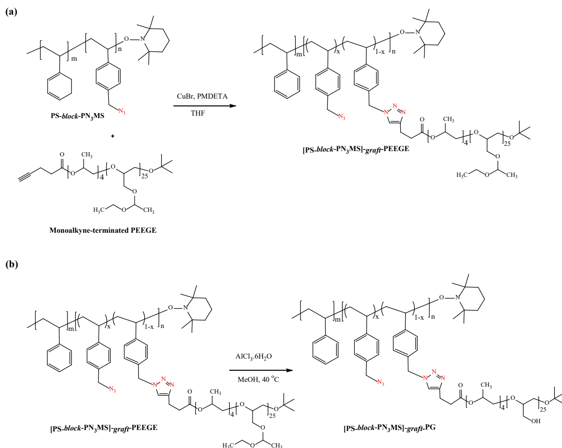
Scheme 1. Schematic representation of the (a) synthesis of [PS- block -PN 3 MS]- graft -PEEGE copolymer by copper-catalyzed click coupling reaction and (b) subsequent deprotection leading to the amphiphilic [PS- block -PN 3 MS]- graft -PG copolymer.
