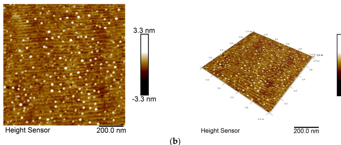
Figure 5. Representative AFM images of micelles deposited from 1 mg/mL aqueous solution: (a) [P(S- ran -N 3 MS)]- graft -PG; (b) [PS- block -PN 3 MS]- graft -PG.
