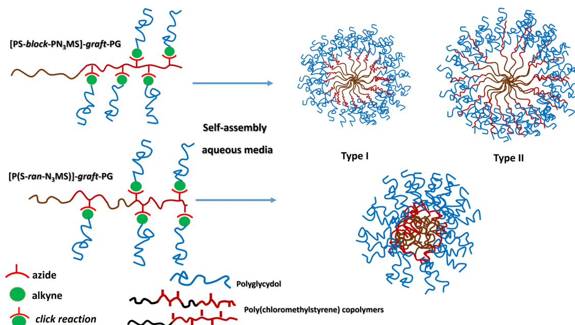
Scheme 2. Schematic representation of the polymeric micelles: models illustrating two types (I and II) of micelle assembly of the coil-comb [PS- block -PN 3 MS]- graft -PG copolymer; model illustrating micelle assembly of the comb-like [P(S- ran -N 3 MS)]- graft -PG copolymer.
