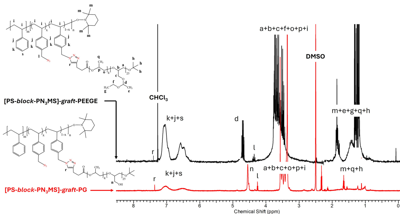
Figure 2. ^1\text{H} NMR spectra of the [PS- block -PN 3 MS]- graft -PEEGE in CDCl 3 and [PS- block -PN 3 MS]- graft -PG in DMSO- d 6 (600 MHz).
