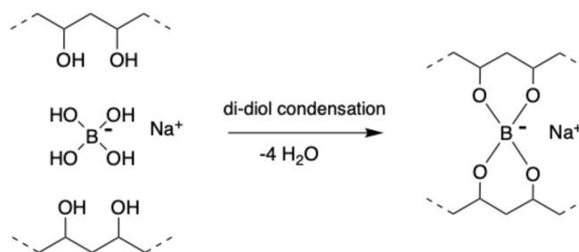
Figure 6. Synthesis of the PVA–borax reversible hydrogel.
