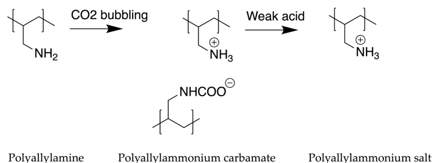
Figure 9. Synthesis of polyallylamine organogels [100].
