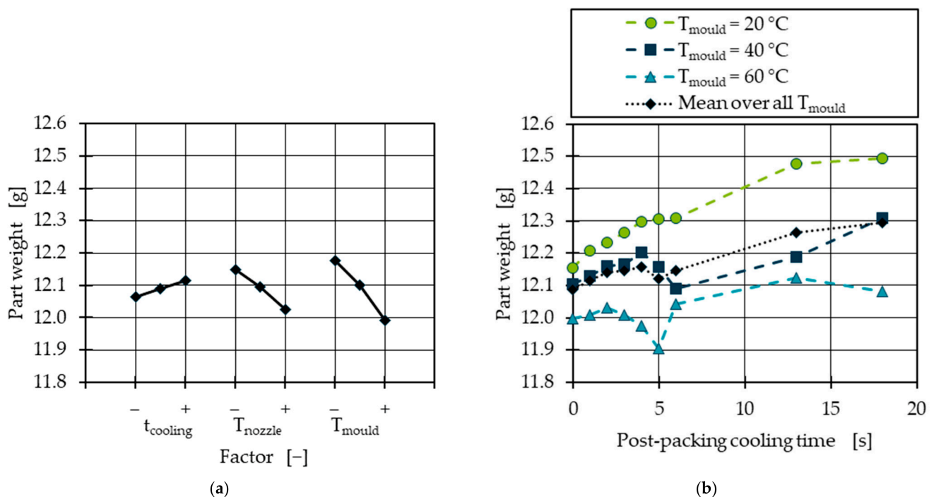
Figure 4. (a) Main effects plot showing the influence of post-packing cooling time ( t_{cooling} ), nozzle temperature ( T_{nozzle} ) and mould temperature ( T_{mould} ) on part weight made from recycled material. (b) Influence of post-packing cooling time and mould temperature on part weight for virgin material.
