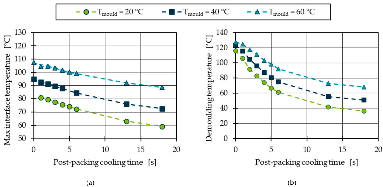
Figure 3. (a) Maximum melt-to-mould interface temperature and (b) demoulding temperature for the virgin polypropylene material at the three mould-temperature settings.
