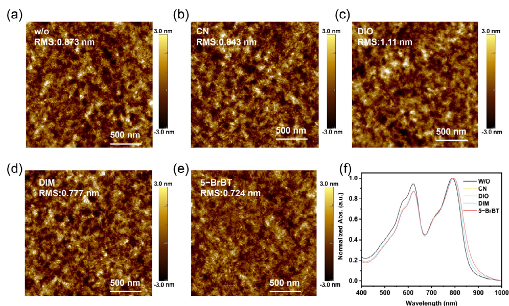
Figure 2. AFM height images of (a) pristine PM6:L8-BO film and PM6:L8-BO film with (b) CN, (c) DIO, (d) DIM, and (e) 5-BrBT as additive, respectively. (f) Absorption spectra of different active layers.
