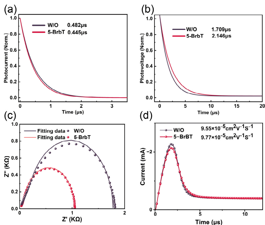
Figure 7. (a) TPC decay curves, (b) TPV relaxation dynamics, (c) Nyquist plots, and (d) Photo-CELIV results of the devices based on the pristine film and the film with 5-BrBT as additive.
