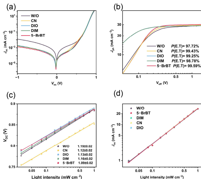
Figure 6. (a) Dark-current curves, (b) J_{ph} - V_{eff} curves, and light intensity-dependent characteristics of (c) V_{oc} and (d) J_{sc} of the OSCs based on pristine PM6:L8-BO films and films with CN, DIO, DIM, and 5-BrBT as additives.
