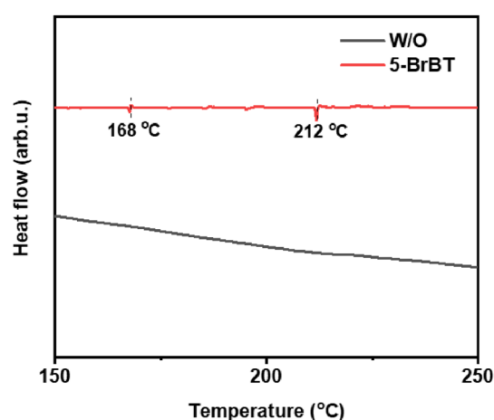
Figure 4. DSC curves of the PM6:L8-BO blend films without additive and with 5-BrBT as the solid additive.
