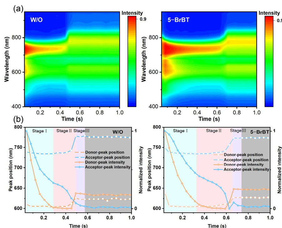
Figure 3. (a) 2D in situ UV-Vis absorption spectra, (b) quantitative evolution curves of absorption peak position and intensity for PM6:L8-BO blend films without additive and with 5-BrBT as the solid additive.
