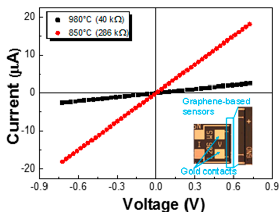
Figure 1. I-V characteristics of the graphene-based resistors reported in the inset.
