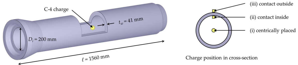
Figure 1. The concrete pipe geometry and a spherical centrally placed charge are shown on the left, while the cross-section and the three different charge positions are shown on the right.
