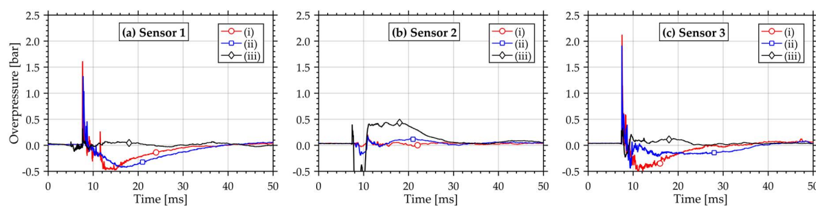
Figure 4. Pressure-time histories from tests with charge size 10.0 g at positions (i), (ii) and (iii), where part (a) shows data from sensor 1, part (b) from sensor 2, and part (c) from sensor 3.
