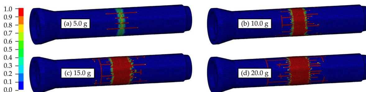
Figure 5. Tensile damage pattern from numerical simulations of blast loaded concrete pipes using charge position (i), where the charge size is (a) 5.0 g, (b) 10.0 g, (c) 15.0 g, and (d) 20.0 g.
