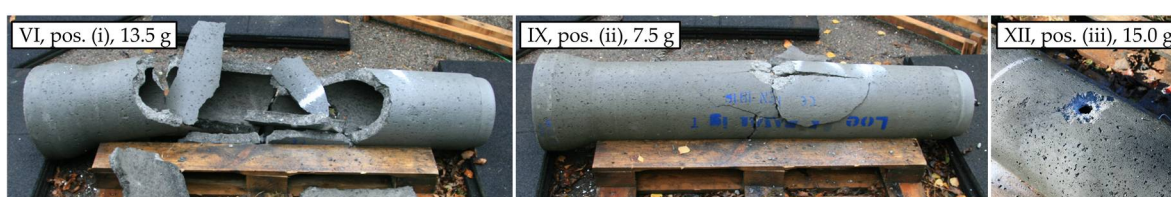
Figure 3. General damage pattern from the three charge positions: (i) left, (ii) centre, and (iii) right.
