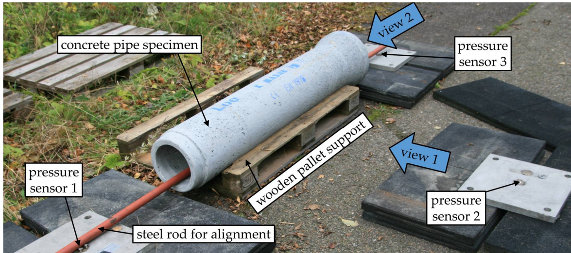
Figure 2. Picture of the experimental setup.
