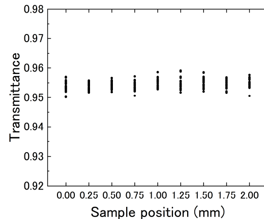
Figure 4. Measured transmittance of the PET sample at each sample position.
