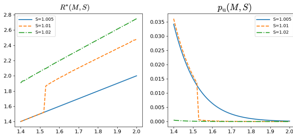
Figure 2. Plots of system behavior as a function of M for fixed lognormal distribution parameters of \mu = 0.033 and \sigma = 0.2 and various values of S . (Left) Agent’s optimal collateral ratio R^*(M, S) with respect to M . Note that when S is low, the agent’s optimal action is to set R = M , but that larger values of S render other, less-risky collateral ratios optimal. (Right) Probability of undercollateralization p_u(M, S) with respect to M . Several features are of note here: first, when S = 1.02 , the probability of undercollateralization is extremely low, despite the fact that only a 2% penalty is assessed the agent in the event of a margin call. Second, when S \leq 1.01 , the probability of undercollateralization ( p_u ) is sharply dependent on the value of M , can be as high in these simulations as 3.5%, and for S = 1.01 , p_u is discontinuous around M = 1.53 . That is, the probability of undercollateralization is extremely sensitive to the operator’s selection of M .
