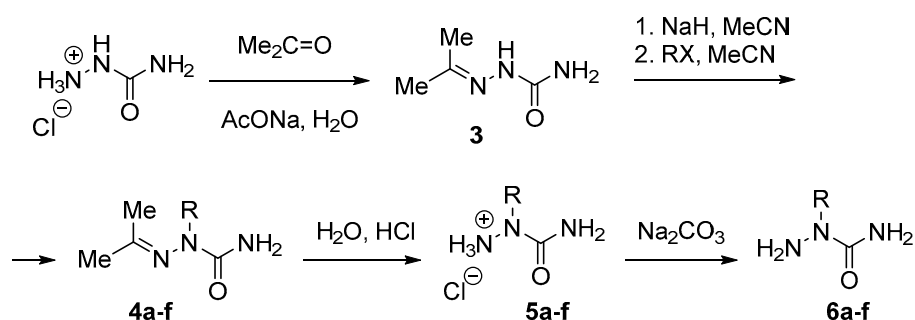
4-6 a R = Me, b R = Et, c R = Pr, d R = Bu, e R = CH 2 Ph, f R = n -C 8 H 17 .
