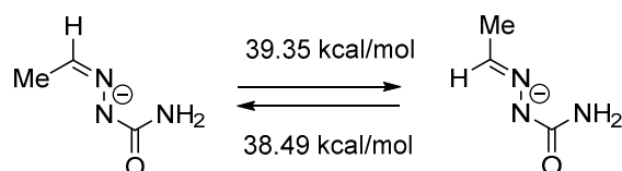
Scheme 3. Transformation of the ( Z )-isomer of the conjugated base of ethanal semicarbazone into the ( E )-isomer via inversion pathway.
