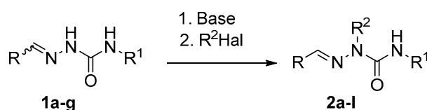
Scheme 2. Synthesis of 2-alkylsemicarbazones by alkylation of 2-unsubstituted semicarbazones.
