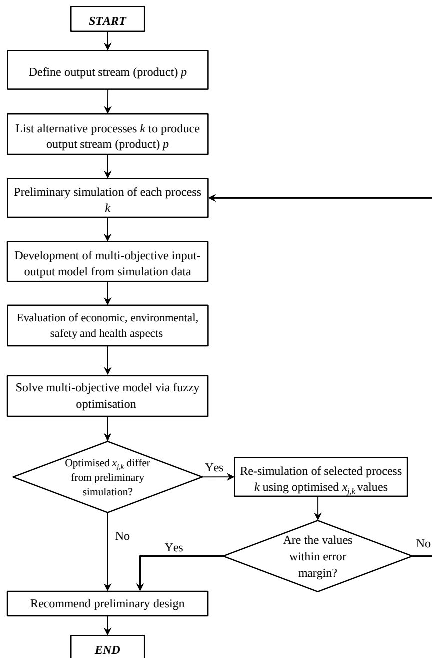
Figure 2. Systematic design framework for preliminary process design.
