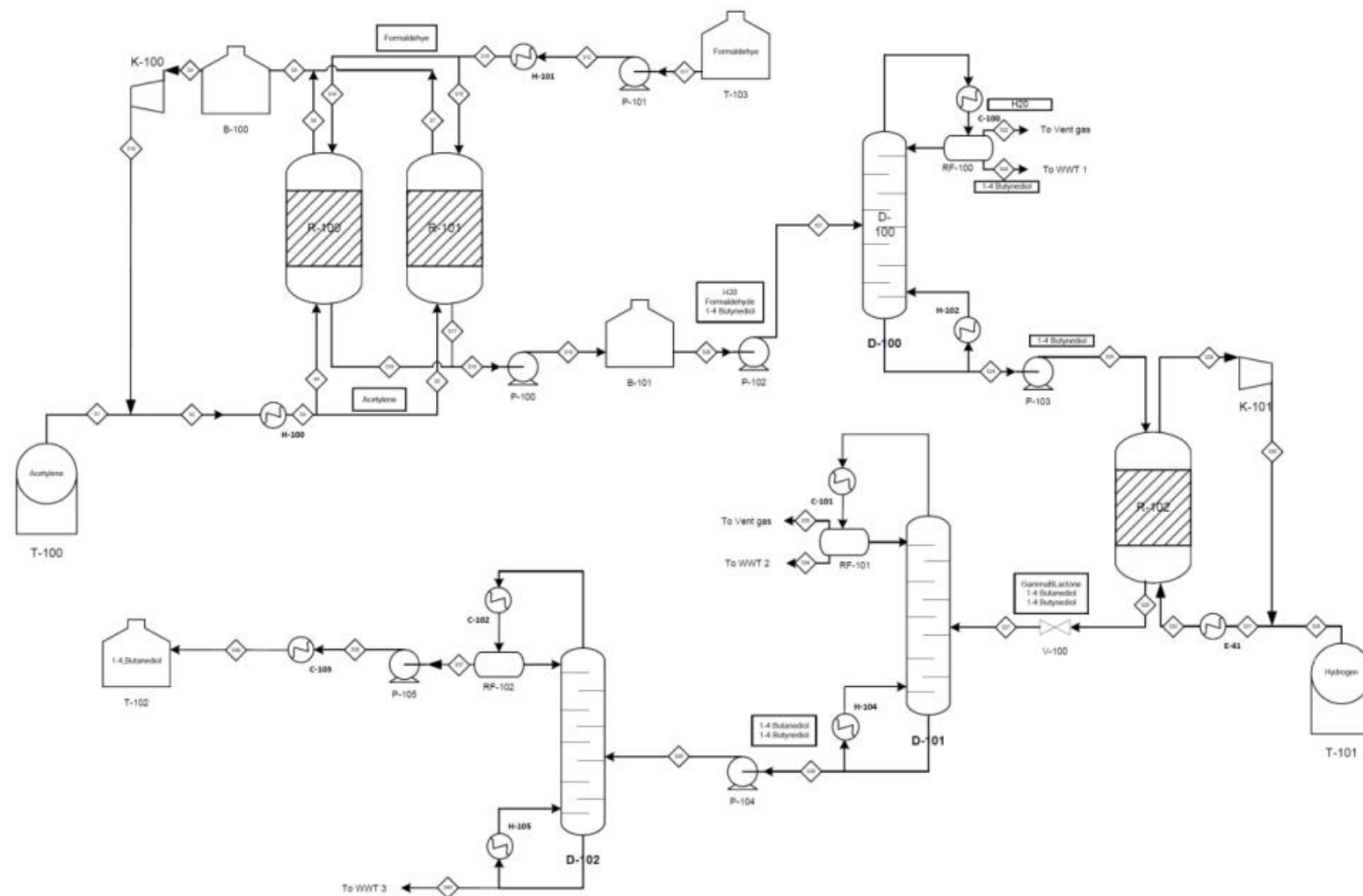
Figure 3. Process flow diagram of the Reppe Process.
