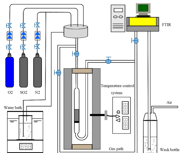
Figure S1 Schematic figure of the fixed bed reactor system for SO 2 adsorption
