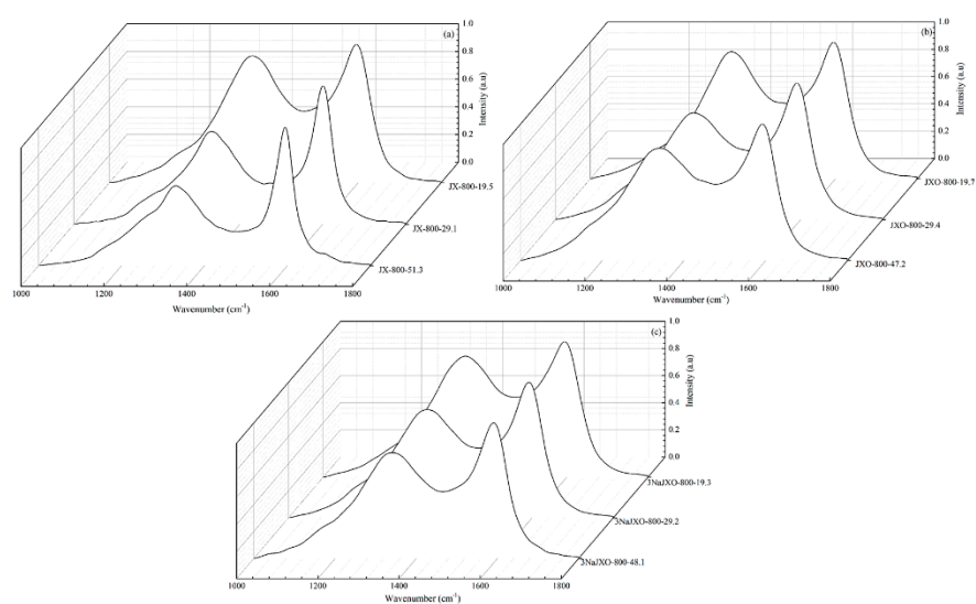
Figure S5. Raman spectra of coal chars at different burn offs during activation (a) JX-800 (b) JXO-800 (c) 3NaJXO-800
