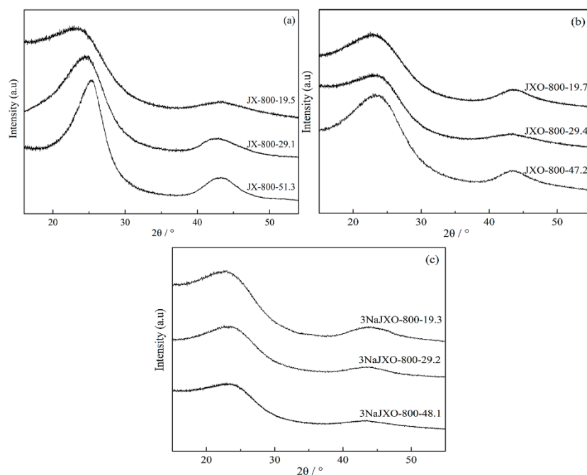
Figure S4. XRD profiles of coal chars at different burn offs during activation (a) JX-800 (b) JXO-800 (c) 3NaJXO-800
