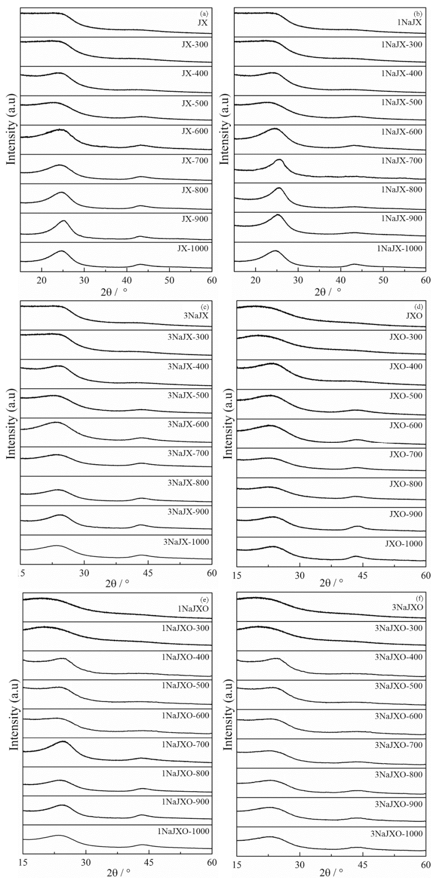
Figure S3 XRD profiles from chars produced by different pyrolysis (a)JX; (b) 1NaJX; (c)3NaJX; (d) JXO; (e) 1NaJXO; (f) 3NaJXO.
