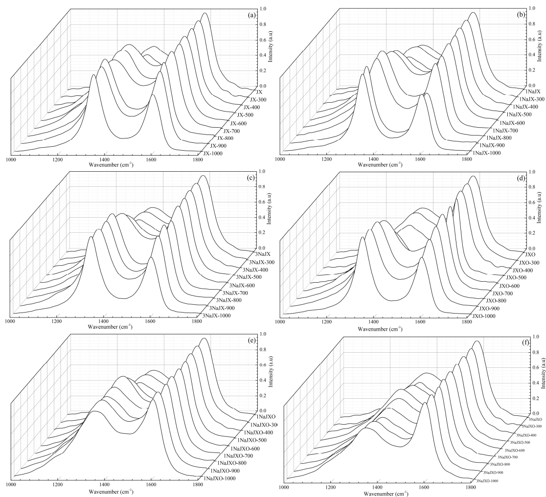
Figure S2 Raman spectra from chars produced by different pyrolysis (a)JX; (b) 1NaJX; (c)3NaJX; (d) JXO; (e) 1NaJXO; (f) 3NaJXO.
