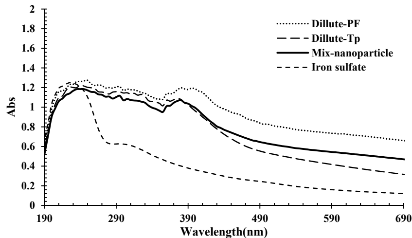
Figure 1. UV-Vis spectra related to the plant extracts, iron solution, and the synthesized nanoparticles.
