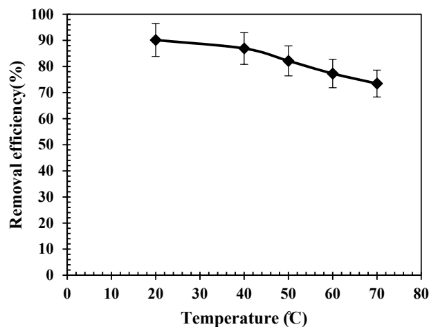
Figure 12. Effect of temperature on arsenic removal efficiency.
