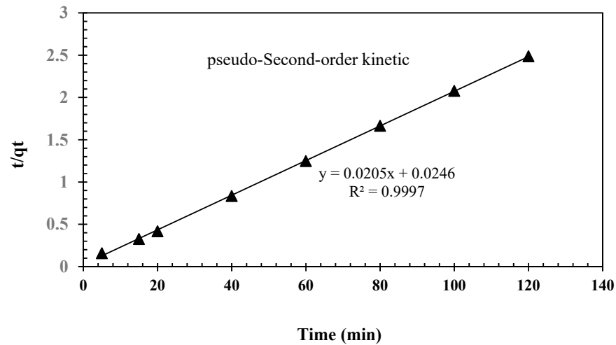
Figure 11. The pseudo-second-order kinetic model for arsenic removal using synthesized iron nanoparticles.
