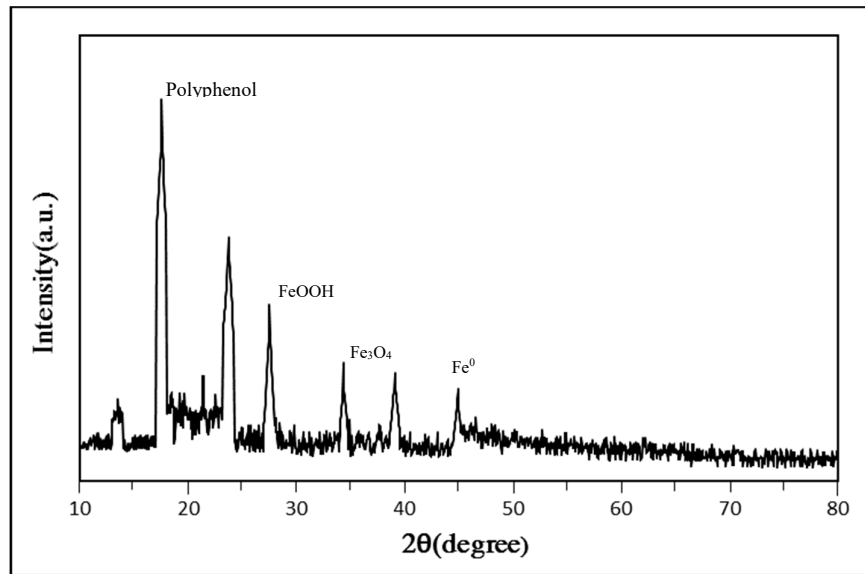
Figure 3. X-ray diffraction (XRD) pattern of synthesized iron nanoparticles from the mixture of extracts.
