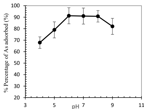
Figure 5. Effect of pH solution on the arsenic removal efficiency (initial arsenic concentration: 0.075 g/L; sorbent dosage: 2 g/L; agitation rate: 150 rpm; time: 15 min).
