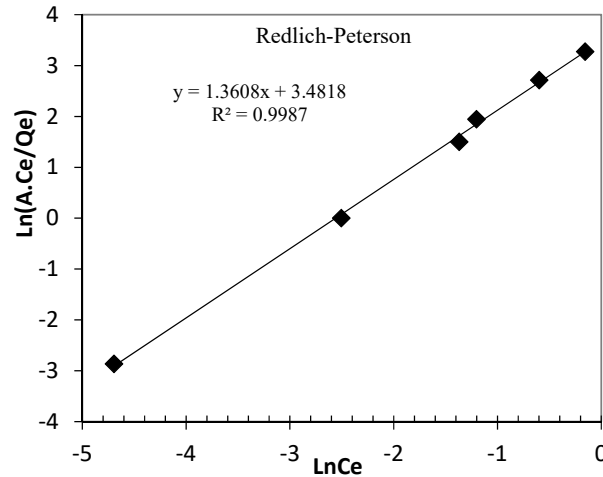
Figure 10. The linearized Redlich–Peterson isotherm model for arsenic sorption onto iron nanoparticles.
