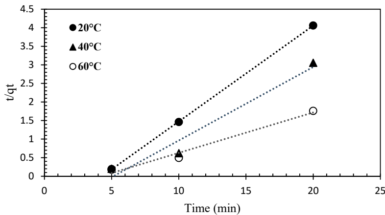
Figure 14. Kinetics of arsenic adsorption at three different temperatures.
