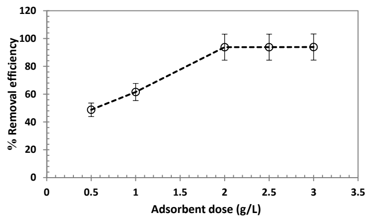
Figure 8. Effect of adsorbent dosage on arsenic removal efficiency (initial arsenic concentration: 0.075 g/L, contact time: 20 min, agitation rate: 150 rpm, pH = 6).
