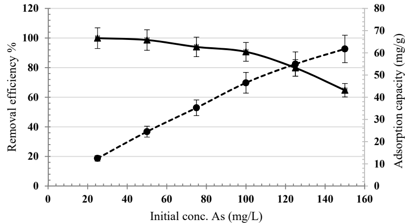
Figure 9. Effect of initial arsenic concentration on arsenic removal efficiency (sorbent dosage: 2 g/L, contact time: 20 min, agitation rate: 150 rpm, pH = 6).
