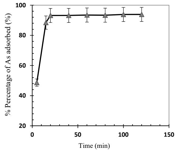
Figure 6. Effect of contact time on arsenic removal efficiency (initial arsenic concentration: 0.075 g/L, sorbent dosage: 2 g/L, agitation rate: 150 rpm, pH = 6).
