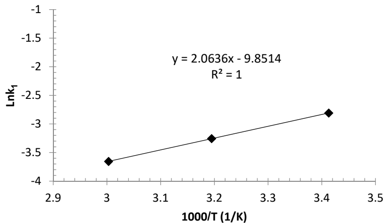
Figure 15. The \ln k_l variations versus 1000/T .
