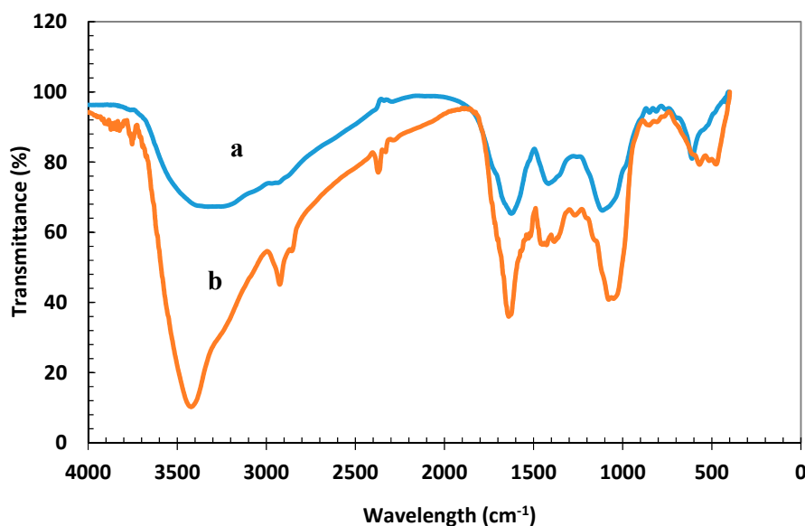
Figure 2. Fourier-transform infrared spectroscopy (FTIR) spectrum of iron nanoparticles (NPs) (a) before and (b) after the adsorption process (resolution = 4, scan times = 10).
