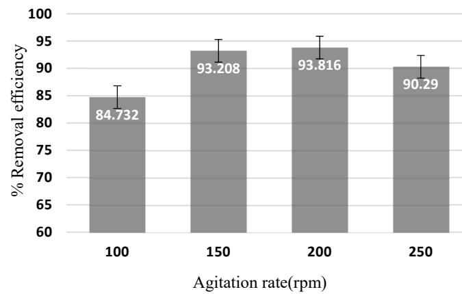
Figure 7. Effect of agitation rate variation on arsenic removal efficiency (initial arsenic concentration: 0.075 g/L, sorbent dosage: 2 g/L, contact time: 20 min, pH = 6).
