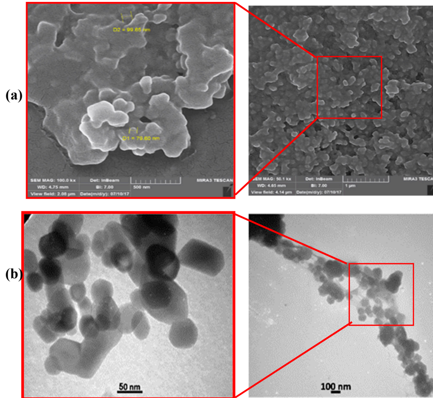
Figure 4. Field emission scanning electron microscopy (FESEM) analysis of synthesized iron nanoparticles at two different magnifications. (a) Transmission electron microscopy (TEM) micrograph of iron exposed by a mixture of extracts (b).
