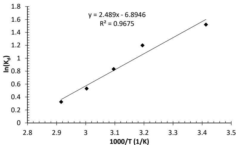
Figure 13. The van't Hoff plot for adsorption of arsenic onto iron nanoparticles.
