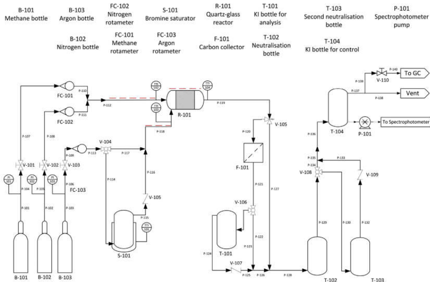
Figure 8. Schematic representation of methane oxidation in bromine mediated processes for energy and coke production. Reprinted from [94].
