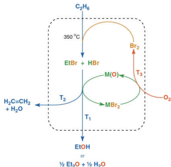
Figure 4. An example of a multi-step process involving halogenation—generation of ethanol or diethyl-ether from ethane. Reproduced from [72] with permission from the Centre National de la Recherche Scientifique (CNRS) and The Royal Society of Chemistry.
