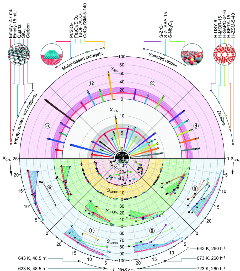
Figure 1. Methane bromination reactions at T = 643\text{ K} and \text{GHSV} (gas hourly space velocity) = 260\text{ h}^{-1} (a) in empty reactors and over supports, (b) supported metal-based catalysts, (c) sulfated oxides, and (d) zeolites. Selectivity to different products in methane bromination (e) in empty reactors and over supports, (f) supported metal-based catalysts, (g) sulfated oxides, and (h) zeolites as a function of methane conversion, which was adjusted by varying the temperature or \text{GHSV} . Conversions and selectivities are expressed in %. Other conditions: \text{CH}_4/\text{Br}_2 = 8.5/3.2 \pm 0.1 and P = 100\text{ kPa} . Reprinted from [40], with the permission of the Royal Society of Chemistry, copyright 2019.
