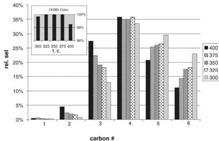
Figure 5. Products of methane bromination and coupling over Ca/ZSM-5 at different temperatures. Carbon numbers 1–4 are predominantly olefins (with trace amounts of alkanes), while 5 and 6 are a mixture of alkanes and alkenes. Reproduced with permission from [74].
