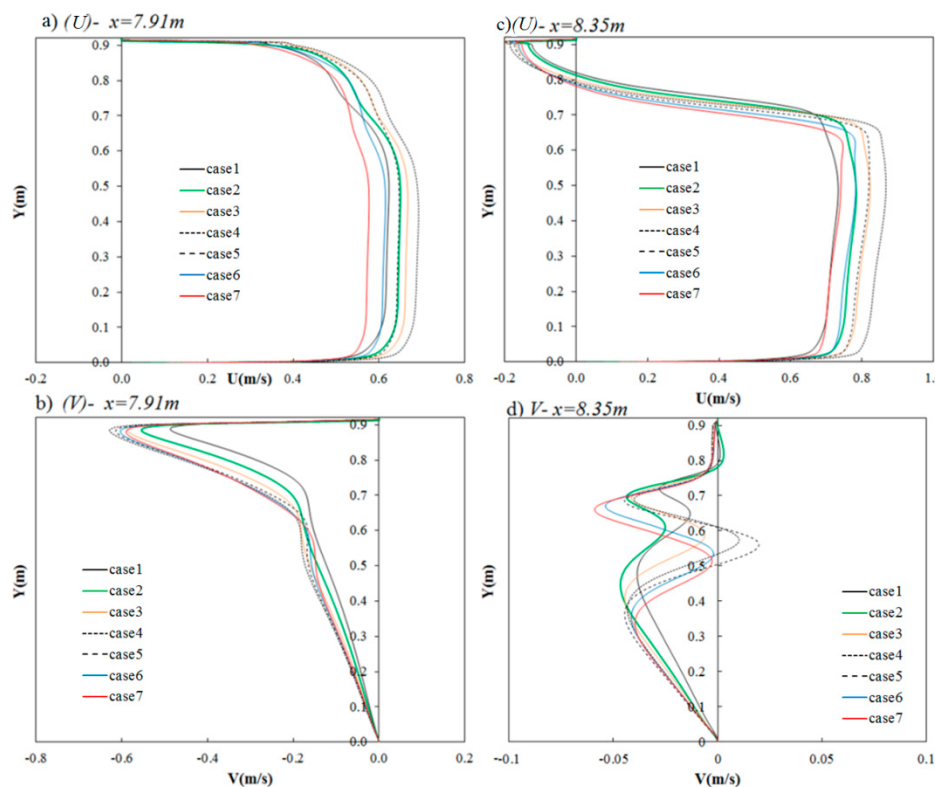
Figure 6. The comparison of velocity components at transverse planes (a) U at x = 7.91 , (b) V at x = 7.91 , (c) U at x = 8.35 m, and (d) V at x = 8.35 m.
