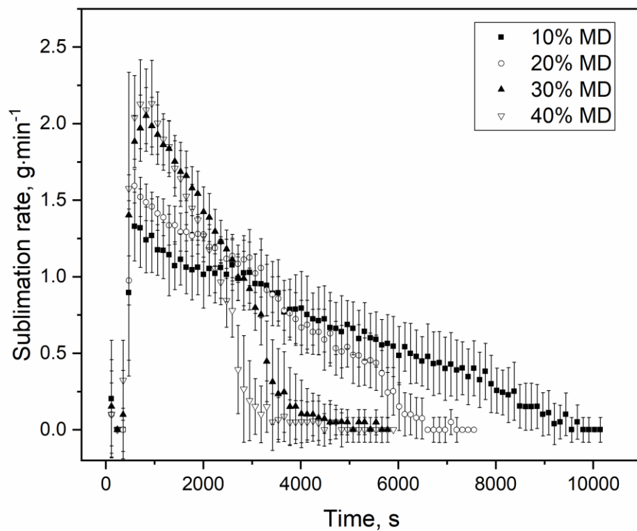
Figure S1. Sublimation rate of foams with MD content between 10 – 40%.
