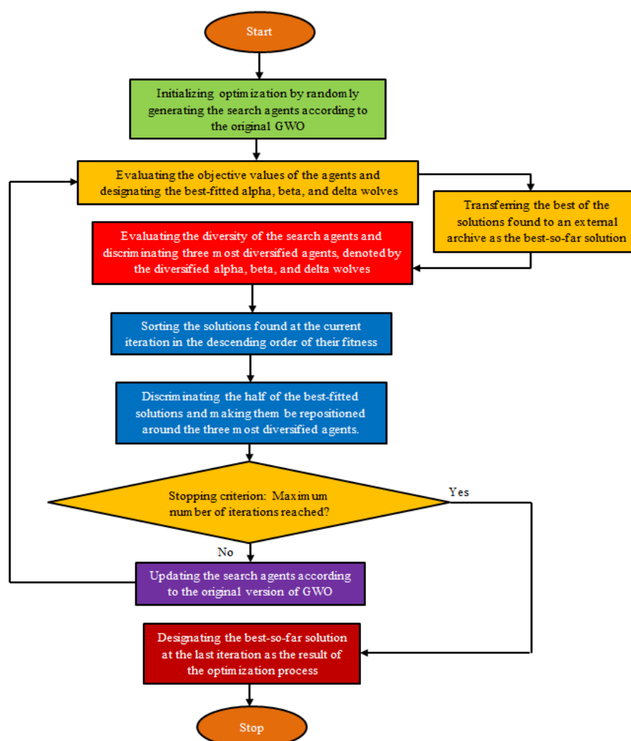
Figure 1. Flowchart of DB-GWO-EPD.
