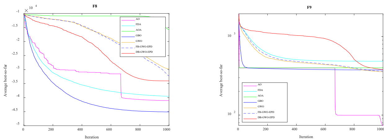
Figure 2. Convergence curves plotted for the algorithms on the uni-modal shifted benchmark functions.
