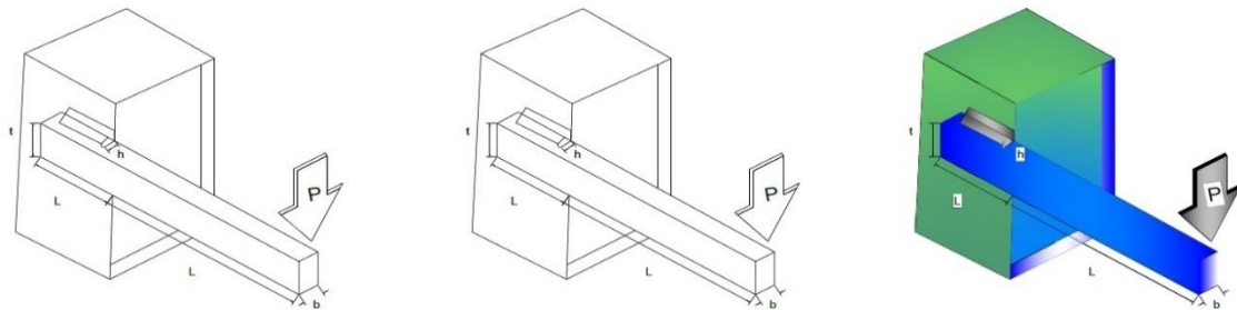
Figure 4. Welded beam scheme [44]. "Reprinted from Publication Reptile Search Algorithm (RSA): A nature-inspired meta-heuristic optimizer, vol. 191, 1–32, Copyright (2022), with permission from Elsevier."
