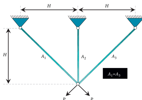
Figure 5. Three-bar truss structure [42].
