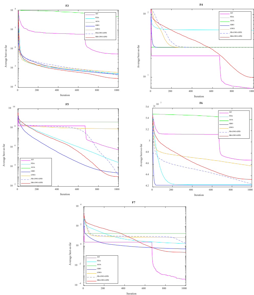
Figure 2. Convergence curves plotted for the algorithms on the uni-modal shifted benchmark functions.
