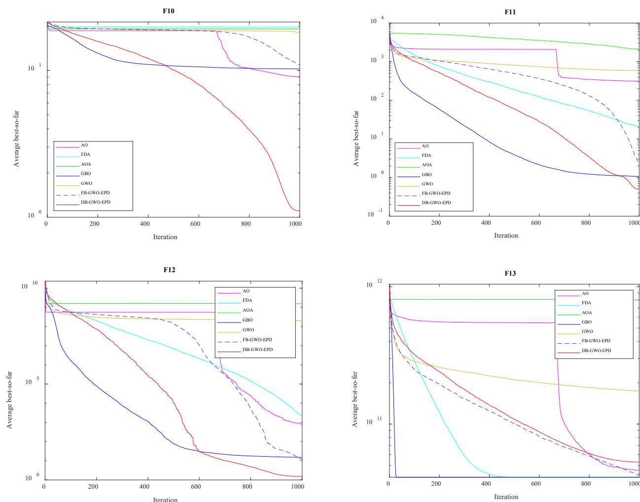
Figure 3. Convergence curves plotted for the algorithms on the multi-modal shifted benchmark functions.
