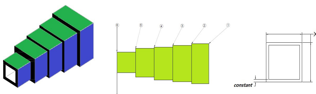
Figure 6. Cantilever beam problem [44]. "Reprinted from Publication Reptile Search Algorithm (RSA): A nature-inspired meta-heuristic optimizer, vol. 191, 1–32, Copyright (2022), with permission from Elsevier."
