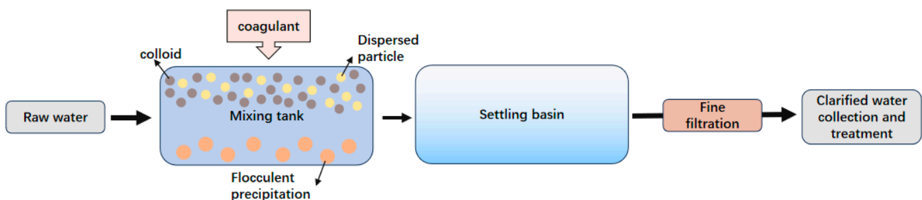
Figure 5. Diagram of the coagulation process.
