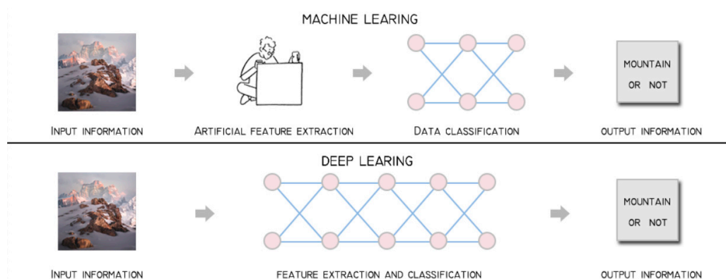
Figure 2. Machine learning vs. deep learning.
