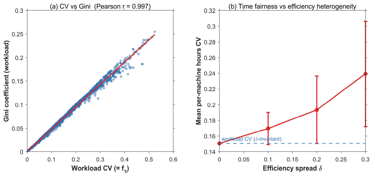
Figure 8. Fairness of the workload-balance objective.
