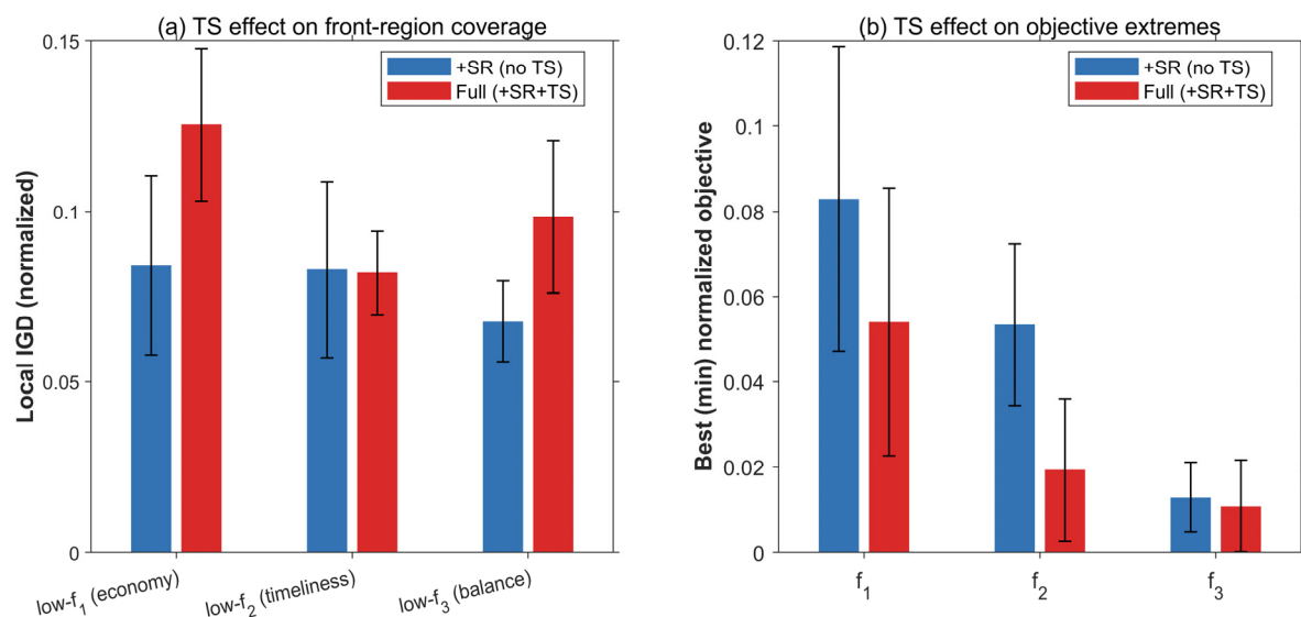
Figure 5. Region- and objective-resolved contribution of Tabu Search on the Liyang instance.
