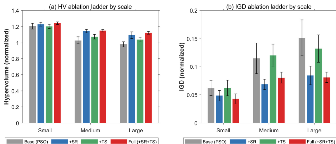
Figure 4. Module-level ablation across the three problem scales.
