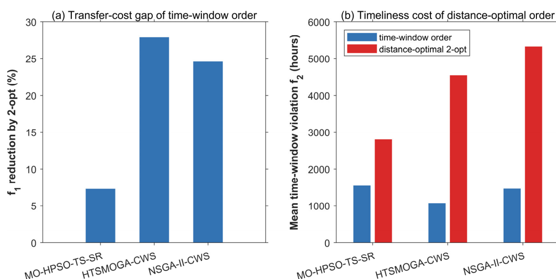
Figure 7. Route-order sensitivity.
