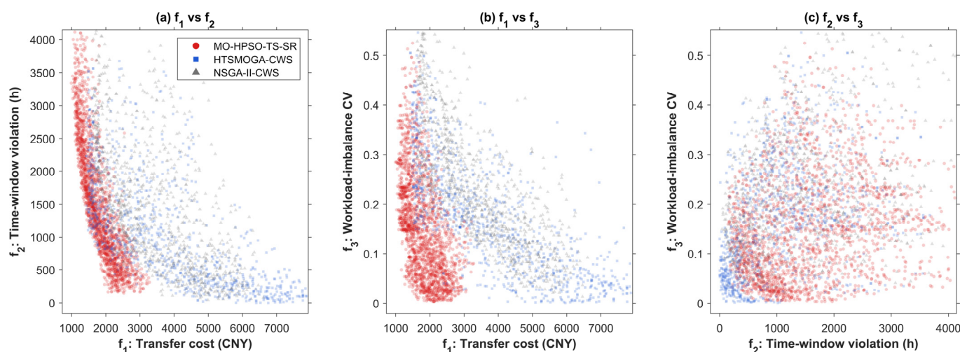
Figure 3. Aggregated Pareto fronts of the three algorithms on the Liyang instance.
