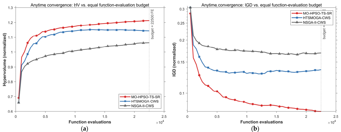
Figure 2. Anytime convergence of the three algorithms on the Liyang instance under the equal 22,500-FE budget: (a) normalized hypervolume and (b) inverted generational distance versus the number of function evaluations.
