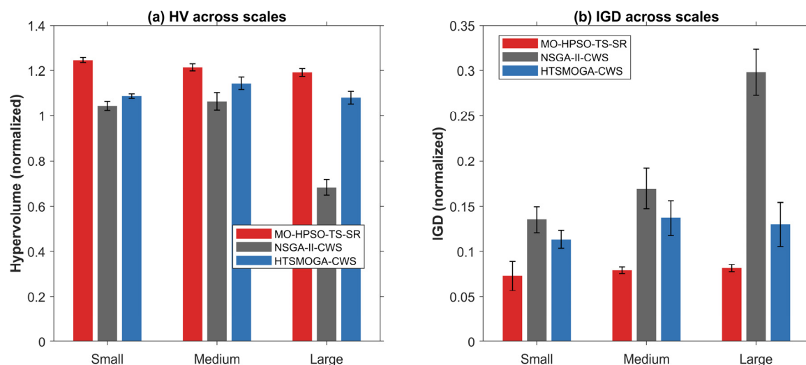
Figure 6. Performance of the three algorithms across problem scales.
