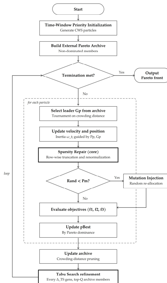
Figure 1. Flowchart of the proposed MO-HPSO-TS-SR algorithm.
