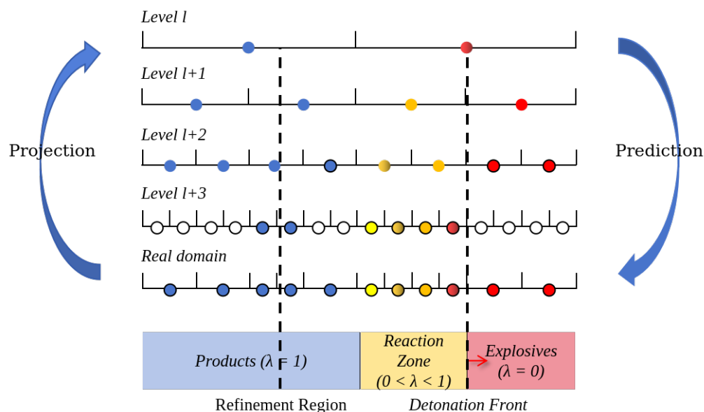
Figure 1. Schematic of the adaptive multi-resolution method for condensed-phase detonation. The arrow indicates the propagation direction of the detonation wave, which moves to the right, with the reaction zone behind it. Circles with black outlines denote leaf nodes, while circles without black outlines denote nodes containing child nodes; filled circles denote valid nodes, and open circles denote empty nodes. The colors distinguish the three regions of the computational domain: product zone (blue, \lambda = 1 ), reaction zone (orange, 0 < \lambda < 1 ), and unreacted explosive zone (red, \lambda = 0 ).
