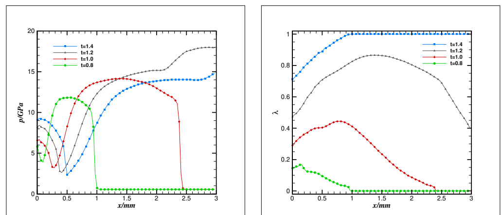
Figure 11. Pressure p (left) and reaction progress variable \lambda (right) distributions along the inner wall at 3 mm for t = 0.8 \mu\text{s} to 1.4 \mu\text{s} .
