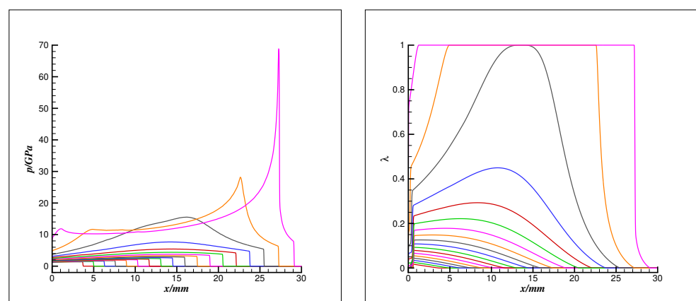
Figure 8. Stage 2: pressure p (left) and reaction progress variable \lambda (right) distributions at t = 0.3 \mu\text{s} to 2.0 \mu\text{s} . Different colored curves denote successive temporal snapshots within this time interval.
