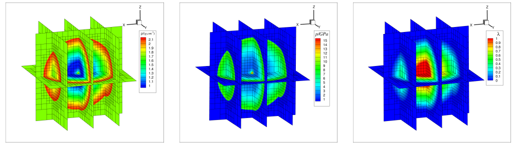
Figure 14. Three-dimensional center-initiation results at t = 1.2 \mu\text{s} . From left to right: density \rho , pressure p , and reaction progress variable \lambda shown on the three orthogonal mid-plane slices ( x = 5 mm, y = 5 mm, and z = 5 mm), with the multi-resolution block structure overlaid in each panel. The adaptive multi-resolution method concentrates refinement near the expanding spherical detonation front.
