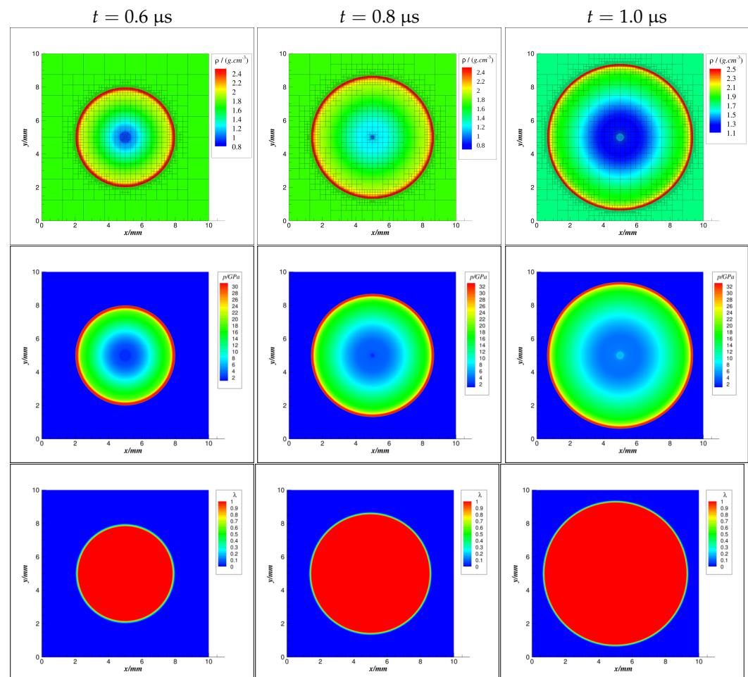
Figure 12. Density (with multi-resolution block structure), pressure, and reaction progress variable distributions from top to bottom at t = 0.6 \mu\text{s} , 0.8 \mu\text{s} , and 1.0 \mu\text{s} from left to right, respectively.
