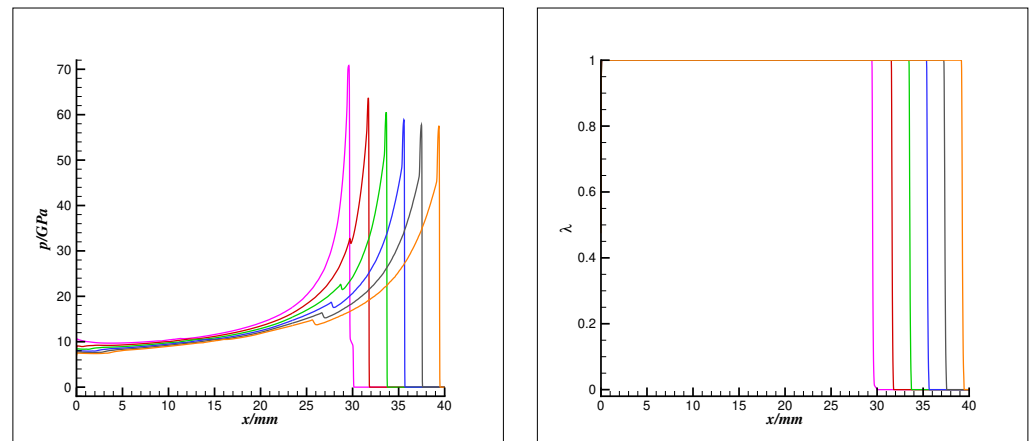
Figure 9. Stage 3: pressure p (left) and reaction progress variable \lambda (right) distributions at t = 2.0 \mu\text{s} to 2.3 \mu\text{s} . Different colored curves denote successive temporal snapshots within this time interval.
