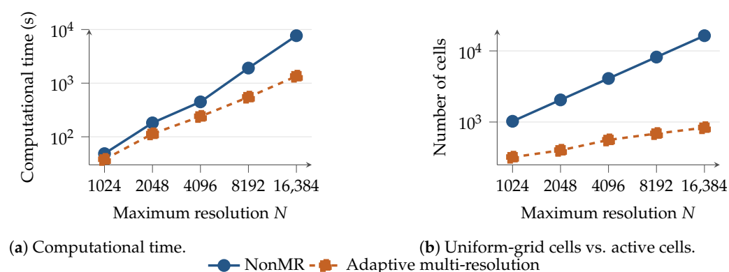
Figure 6. Direct comparison between the uniform-grid (NonMR) and the adaptive multi-resolution computations for the 1D strong-shock initiation benchmark. Both vertical axes are logarithmic.
