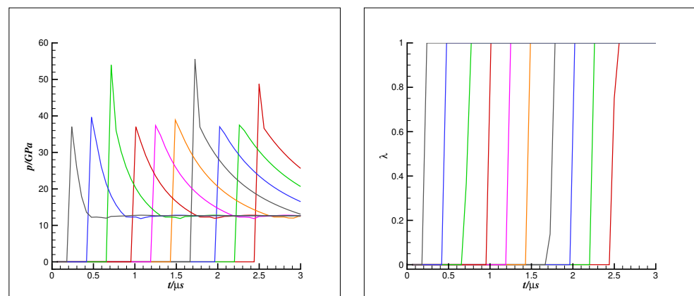
Figure 5. Tracer point histories of pressure p (left) and reaction progress variable \lambda (right) for the 1D strong shock initiation case. Different colored curves denote histories recorded at different tracer-point locations along the propagation direction.
