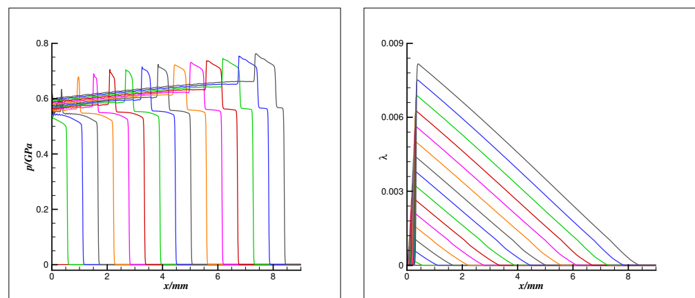
Figure 7. Stage 1: pressure p (left) and reaction progress variable \lambda (right) distributions at t = 0 \mu\text{s} to 0.3 \mu\text{s} . Different colored curves denote successive temporal snapshots within this time interval.
