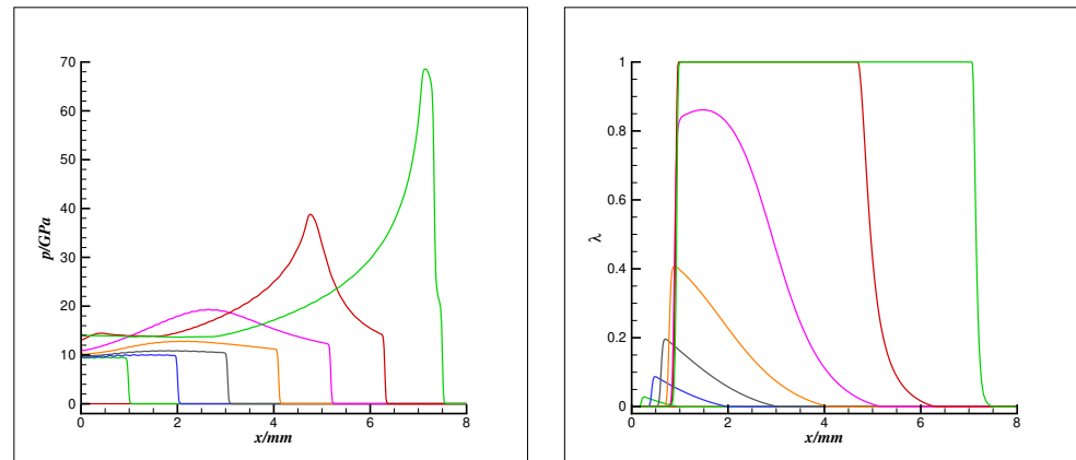
Figure 3. Stage 1: pressure p (left) and reaction progress variable \lambda (right) distributions at t = 0 \mu\text{s} to 0.35 \mu\text{s} with a time interval of 0.05 \mu\text{s} . Different colored curves denote successive temporal snapshots within this time interval.
