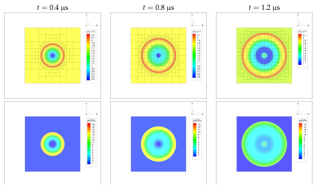
Figure 15. z = 5 mm slice contour maps for the three-dimensional center-initiation case. Top row: density \rho ; bottom row: pressure p . Columns correspond to t = 0.4 \mu\text{s} , 0.8 \mu\text{s} , and 1.2 \mu\text{s} (left to right). The overlapping “Z” label does not affect the scientific interpretation of the contour fields.
