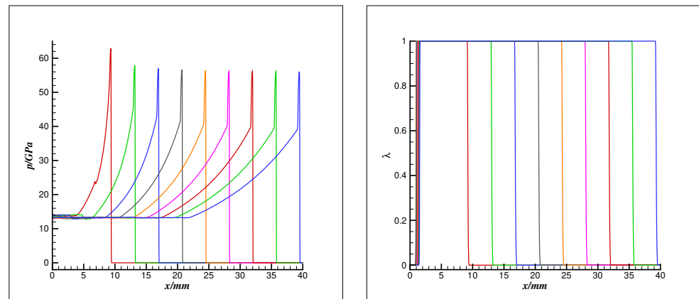
Figure 4. Stage 2: pressure p (left) and reaction progress variable \lambda (right) distributions at t = 0.4 \mu\text{s} to 1.2 \mu\text{s} with a time interval of 0.1 \mu\text{s} . Different colored curves denote successive temporal snapshots within this time interval.
