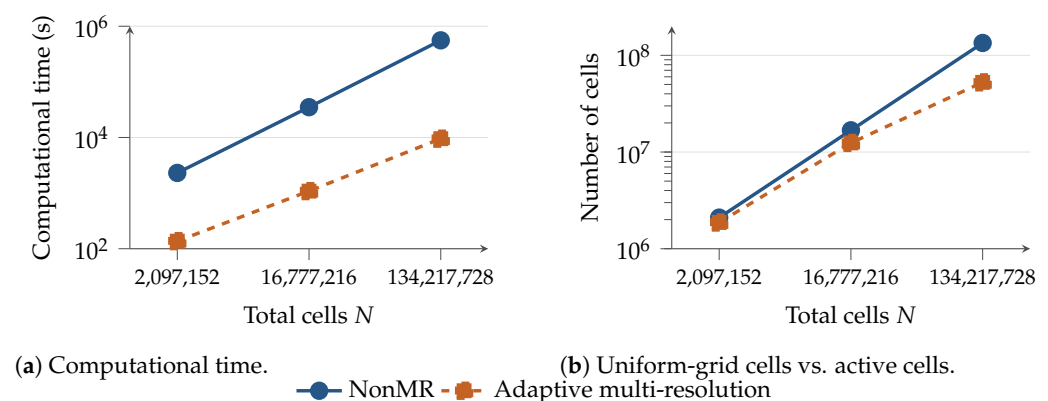
Figure 16. Direct comparison between the uniform-grid (NonMR) and adaptive multi-resolution computations for the 3D center-initiation benchmark. Both vertical axes are logarithmic.
