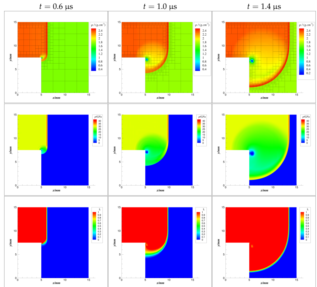
Figure 10. Density (with multi-resolution block structure), pressure, and reaction progress variable distributions from top to bottom at t = 0.6 \mu\text{s} , 1.0 \mu\text{s} , and 1.4 \mu\text{s} from left to right, respectively, for the corner diffraction problem.
