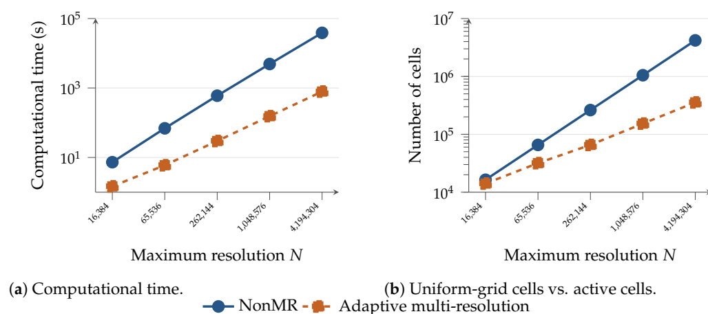
Figure 13. Direct comparison between the uniform-grid (NonMR) and adaptive multi-resolution computations for the 2D center-initiation benchmark. The x-axis tick labels are rotated and comma-separated to improve readability. Both vertical axes are logarithmic.
