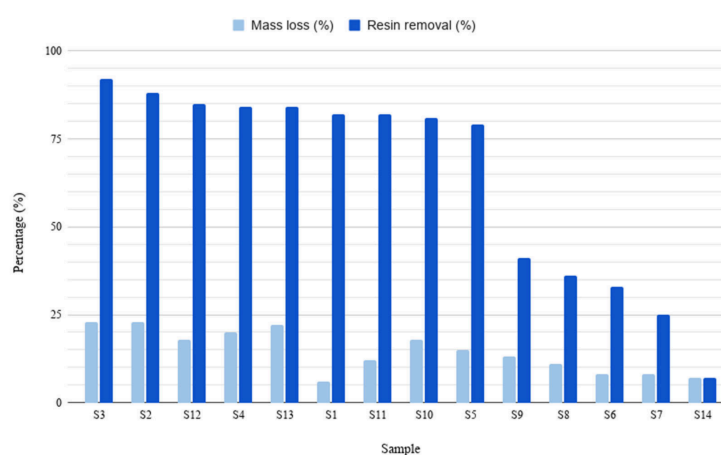
Figure 2. Relationship between mass loss and UF resin removal during steam-assisted hydrolysis.
