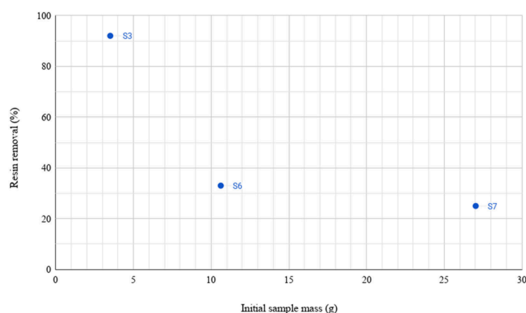
Figure 1. Effect of the initial sample mass on UF resin removal during steam-assisted hydrolysis.
