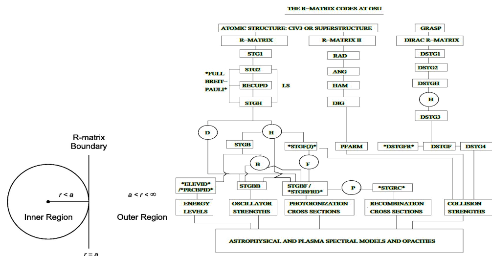
Figure 4. L: R-matrix sphere. R: Algorithm of R-matrix codes. For descriptions, see [1]. * indicates component created at the Ohio State University.
