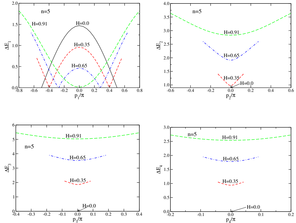
Figure 4. (Color online) Spinwave excitations for n = 5 for several fields ( H = 0 black solid line; H = 0.35 red dashed line; H = 0.65 blue dash-dotted line; H = 0.91 green long-dashed line). ( left top panel ) \Delta E_1 : The Fermi momentum is defined as the zero of \Delta E_1(p_F) for each H . Hole excitations correspond to -p_F < p_1 < p_F , while particle excitations to |p_1| > p_F . The range of p_1 increases with H . For H > 0.91 the excitations are gapped and have no Fermi point. ( right top panel ) \Delta E_2 : The excitation energies are gapped, except for H = 0 , where the dispersion reduces to a single point and all states are empty in this case. ( lower left panel ) \Delta E_3 : For the third band the dispersion again reduces to a point for H = 0 . ( lower right panel ) \Delta E_4 : Similar to \Delta E_2 and \Delta E_3 .
