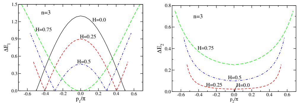
Figure 2. (Color online) Spinwave excitations for n = 3 for several fields ( H = 0 black solid line; H = 0.25 red dashed line; H = 0.5 blue dash-dotted line; H = 0.75 green long-dashed line). (left panel) \Delta E_1 : The Fermi momentum is defined as the zero of \Delta E_1(p_F) for each H . Hole excitations correspond to -p_F < p_1 < p_F , while particle excitations to |p_1| > p_F . The range of p_1 increases with H . For H > 0.75 the excitations are gapped and have no Fermi point. (right panel) \Delta E_2 : The excitation energies are gapped, except for H = 0 , where the dispersion reduces to a single point. All states are empty in this case.
