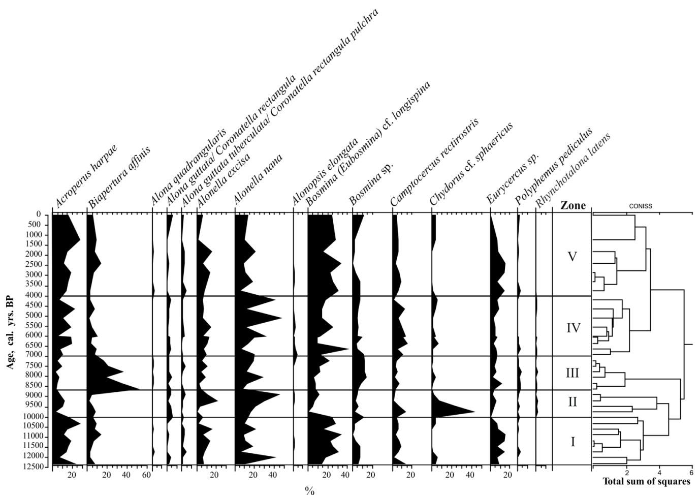
Figure 2. Stratigraphic distribution of statistically significant taxa of Cladocera in the column of bottom sediments of Lake Medvedevskoye and Rhynchotalona latens , Karelian Isthmus, Kola–Karelian region, European Russia. I, II, III . . . are the numbering of faunal zones.
