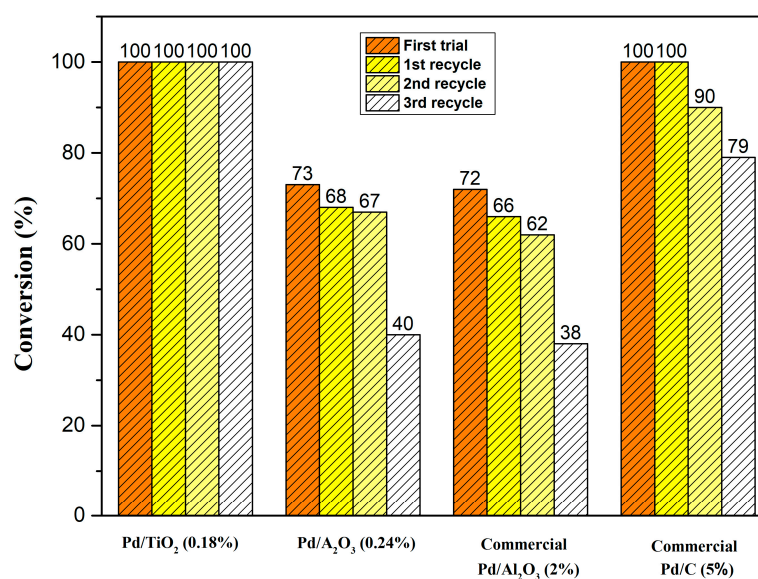
Figure 2. Comparison of catalytic performance of synthesized and commercial supported Pd catalysts in the hydrogenation of (E)-cinnamaldehyde (I).
