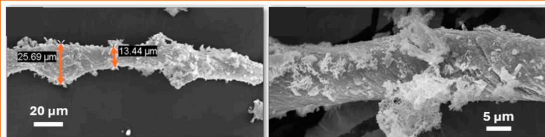
Figure 6. Biomorphic catalytic fibers reported by Rodriguez [94]. (a) Procedure for obtaining catalytic ceramic fibers through biomorphic synthesis. (b) SEM images (different magnifications) of \text{CeO}_2 catalysts deposited on either biomorphic Mn or Co fibers.
