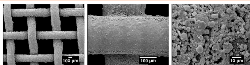
Co-Ce fibers
