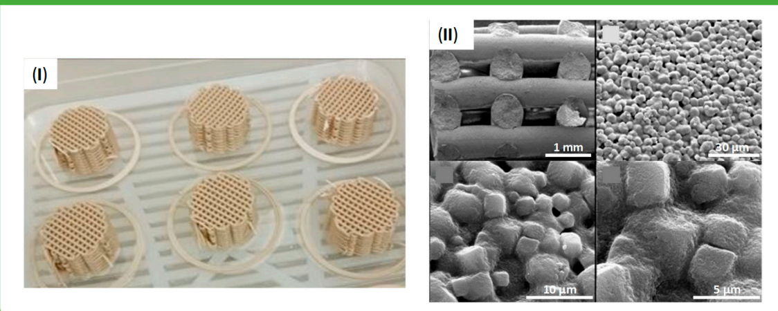
(b) SEM images of 3D-printed microstructures of inorganic porous materials.
