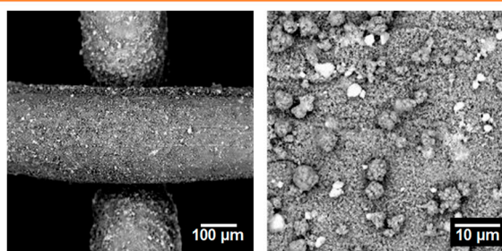
Figure 9. Stainless steel wire mesh monoliths developed by Godoy [113]. (a) Photograph of an un-assembled cartridge showing the inner mesh (left). Assembled metal cartridges containing stainless steel mesh with different mesh sizes (right). (b) SEM images of the central mesh of a cartridge coated with a layer of CeO 2 , onto which Pt (top images) or Co 3 O 4 (bottom images) was impregnated.
