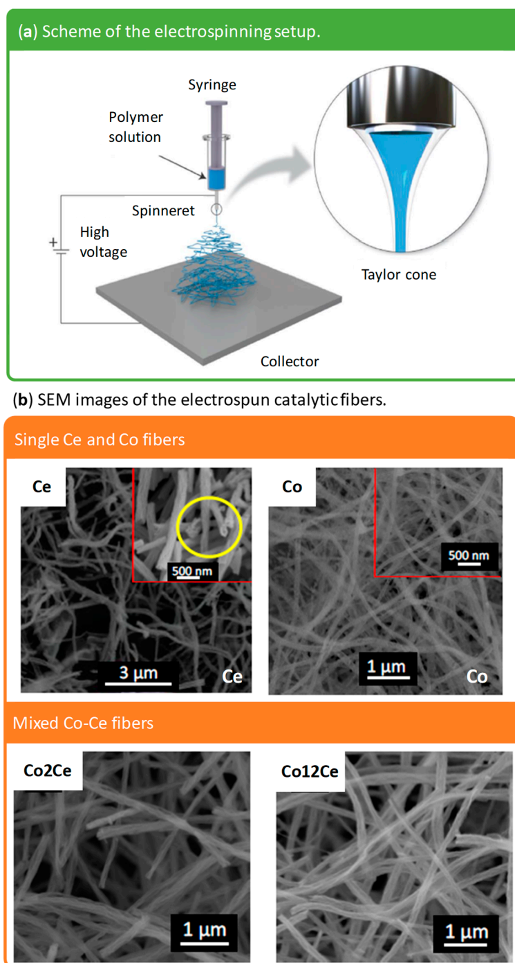
Figure 7. Electrospun fibers synthesized by Stegmayer [100]. (a) Schematic diagram of the device used in the synthesis of ceramic fibers via the electrospinning method. (b) SEM images of bulk electrospun fibers (cerium oxide fibers left and cobalt oxide fibers right) and cobalt-supported cerium oxide fibers with different cobalt loadings: 2 wt.% (left) and 12 wt.% (right). The yellow circle shows that the fibers are hollow.
