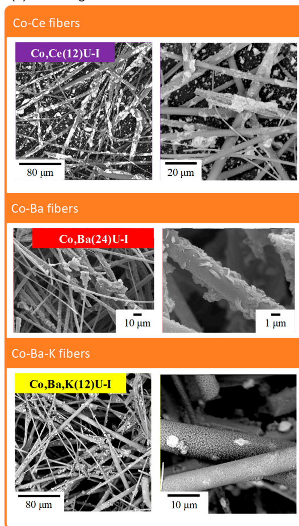
Figure 10. Ceramic fibers structured as ceramic papers [88,116]. (a) Images that show the flexibility and porosity of ceramic papers. (b) Micrographs of \text{SiO}_2\text{--Al}_2\text{O}_3 ceramic papers loaded with either cobalt + cerium, cobalt + barium or cobalt + barium + potassium catalysts.
