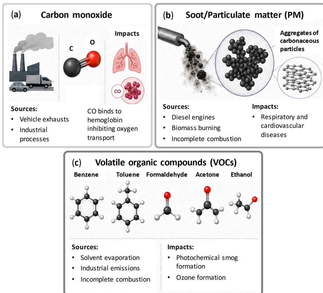
Figure 2 Main atmospheric pollutants relevant to catalytic oxidation. (a) Carbon monoxide, (b) Soot particles and (c) Volatile organic compounds. Ball symbols: carbon (black), hydrogen (white), oxygen (red).
