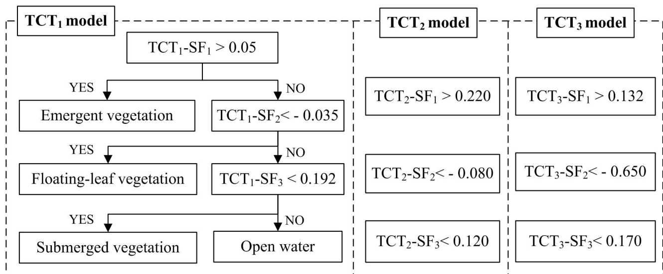
Figure 3. Traditional classification tree (TCT) model structure and thresholds of spectral features (SFs) resulting from the three image dates. TCT 1 model is the model developed for the July image using field data from July (group I). TCT 2 and TCT 3 models were similarly developed for August and September images and their respective ground sample groups (sample groups II and III). TCT 1 -SF 1 , TCT 1 -SF 2 and TCT 1 -SF 3 are SF 1 , SF 2 and SF 3 values (see Table 3) obtained from the July image. TCT 2 -SF 1 , TCT 2 -SF 2 and TCT 2 -SF 3 are SF 1 , SF 2 and SF 3 values obtained from the August image. TCT 3 -SF 1 , TCT 3 -SF 2 and TCT 3 -SF 3 are SF 1 , SF 2 and SF 3 values obtained from the September image.
