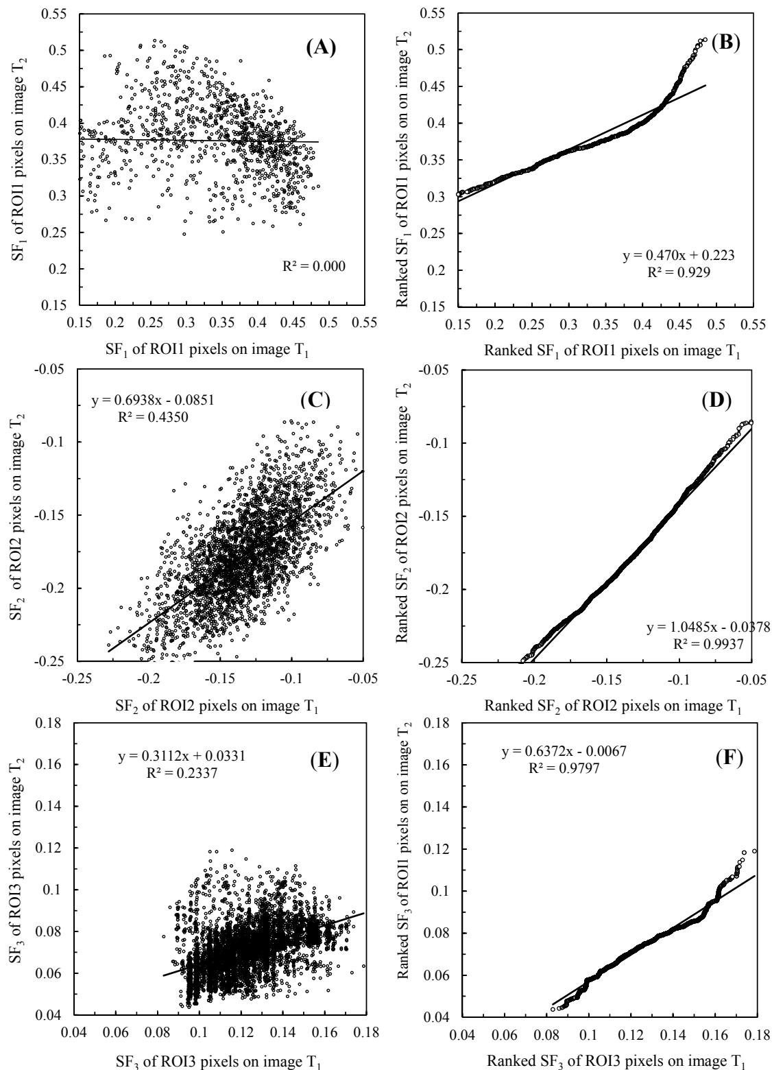
Figure 6. Correlations between Spectral features (SFs) of ROIs for image T_1 (11 July 2013) and image T_2 (16 August 2013) under hypothesis I and hypothesis II. Correlation between SF 1 of ROI 1 for image T_1 and image T_2 under hypothesis I (A) and hypothesis II (B); Correlation between SF 2 of ROI 2 for image T_1 and image T_2 under hypothesis I (C) and hypothesis II (D); Correlation between SF 3 of ROI 3 for image T_1 and image T_2 under hypothesis I (E) and hypothesis II (F). See Table 3 for descriptions of SF 1 , SF 2 and SF 3 ; See Table 4 for descriptions of ROI 1, ROI 2 and ROI 3.
