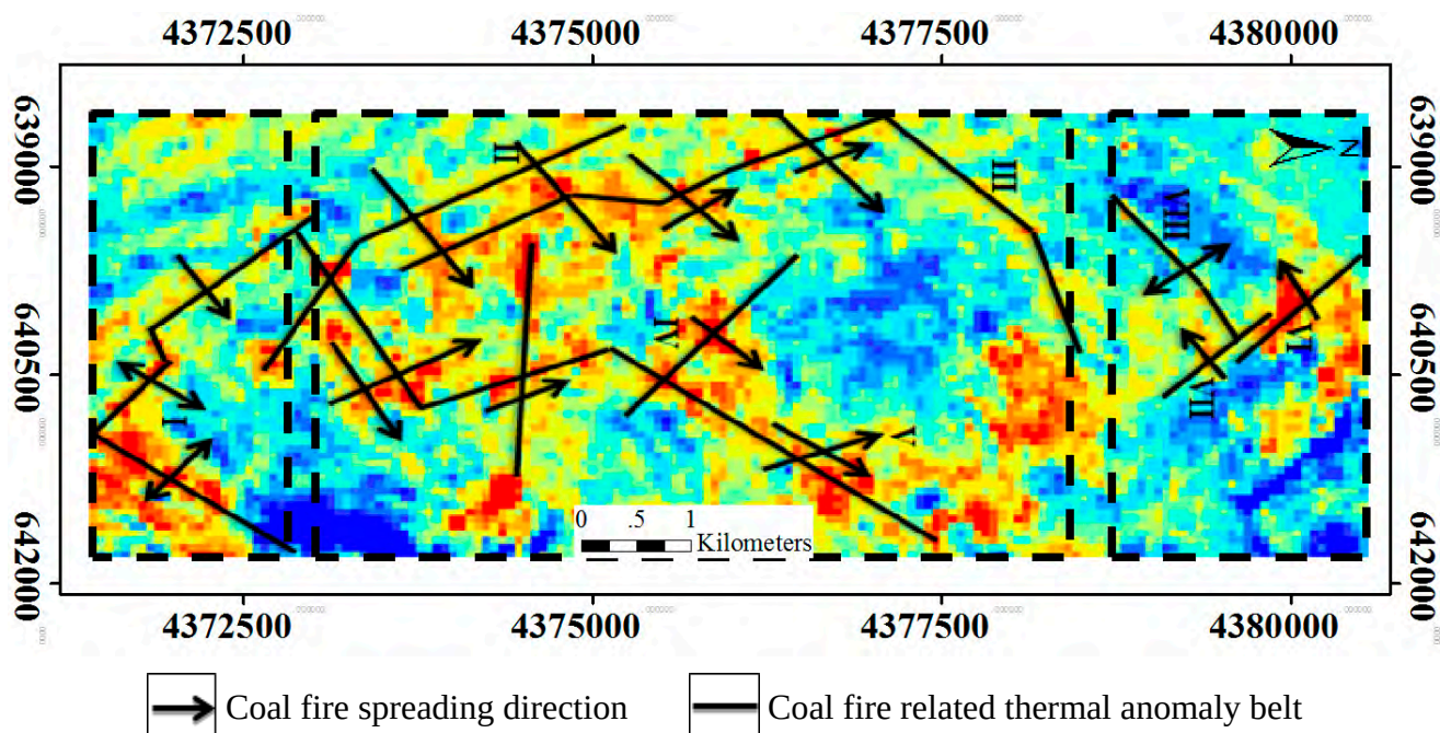
Figure 15. Coal fire spreading direction predicted based on the coal fires that were extracted from long-time series satellite data (See Figure 11) and the base map was 1999 Landsat ETM+ thermal band 6 data, which was sliced with the color table using the ENVI software. The lines of the coal fire spreading direction were drawn using ArcGIS software.
