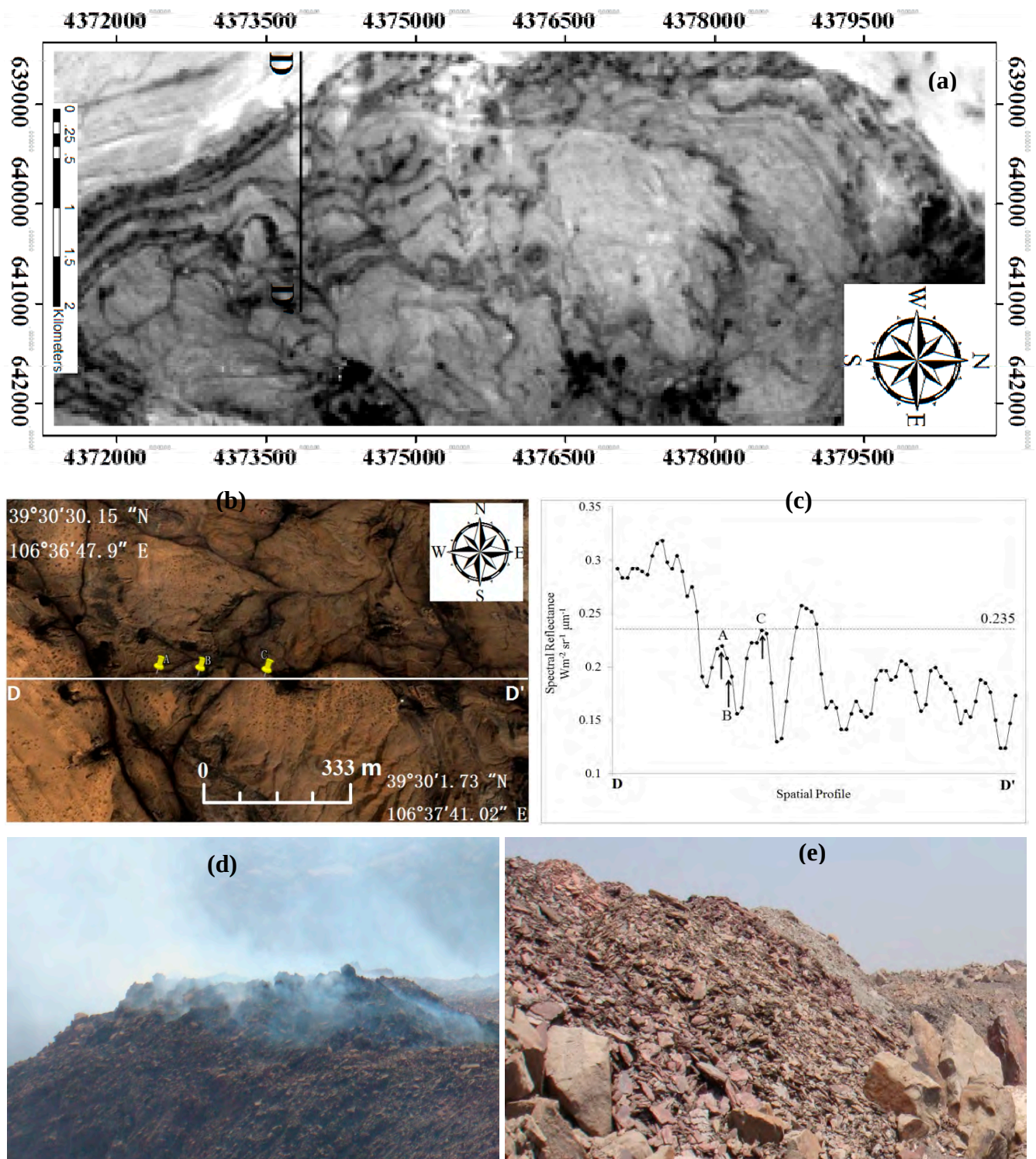
Figure 7. The methodology that was followed in the study to remove coal overburden wastes is presented here with a thresholding method using the WCF as an example. (a) The location of the selected profile line DD' on Landsat TM band-7 image of 3 May 2003; (b) Underground coal fire location A and B and coal overburden dump location C along the selected spatial profile DD' are shown as a reference on a very high resolution Google Earth TM back ground image of 5 October 2003; (c) Maximum reflectance along the spatial profile line DD'; (d) Field photograph of a coal fire location B; (e) Field photograph of a coal overburden dump at location C.
