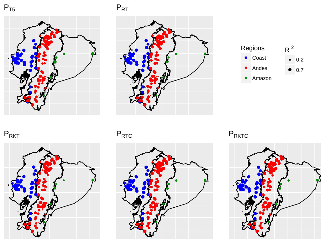
Figure 9. R^2 of the five products over the station points.
