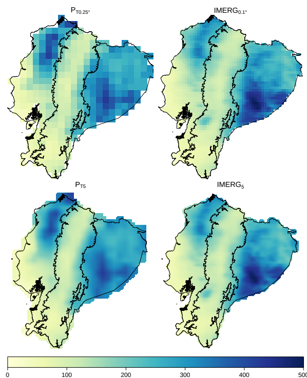
Figure 10. Monthly precipitation [mm] of April 2014 for the TRMM product and IMERG, both at their native resolution and resampled to 5 km.
