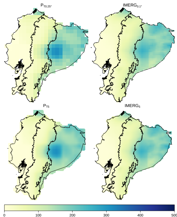
Figure 11. Monthly precipitation [mm] of August 2014 for the TRMM product and IMERG, both at their native resolution and resampled to 5 km.
