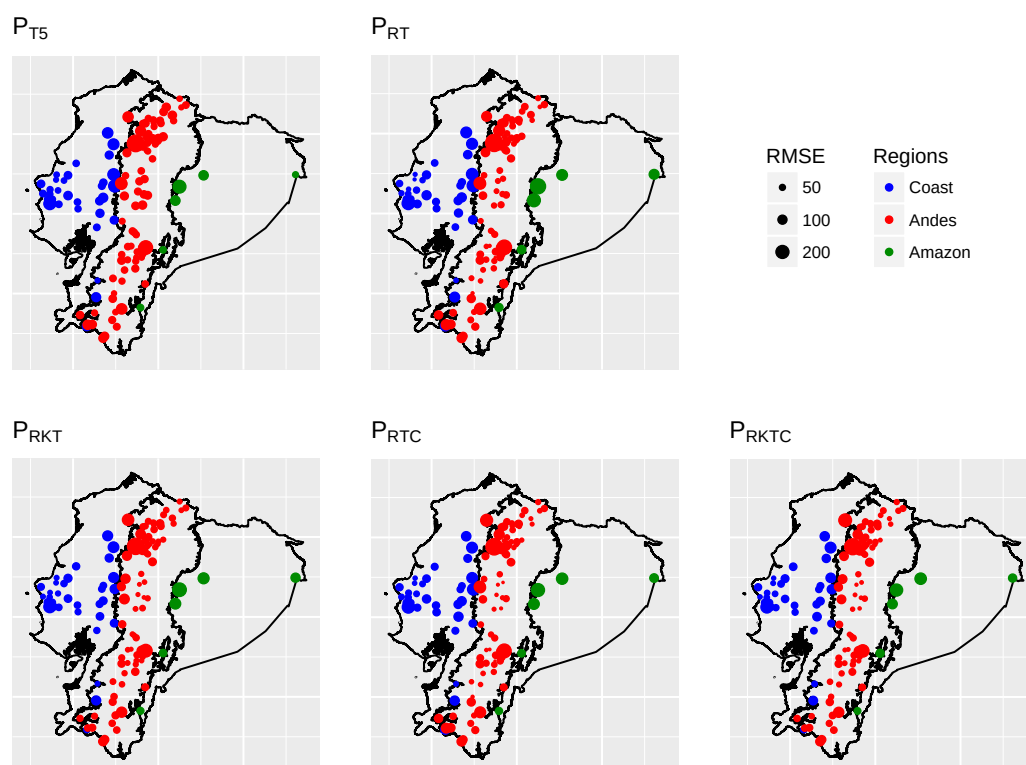
Figure 7. RMSE of the five products over the station points.
