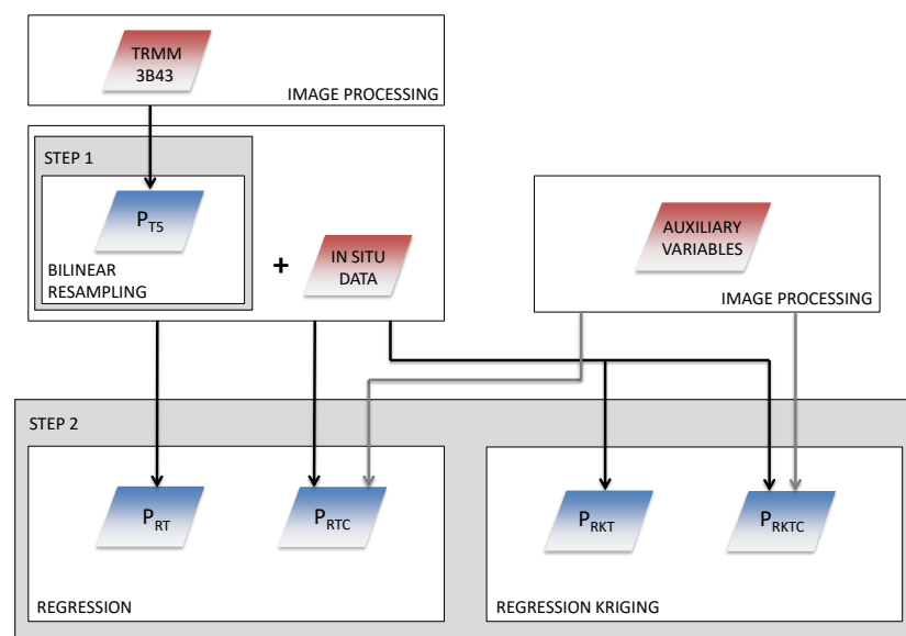
Figure 2. Work flow of the overall downscaling procedure and the 5 resulting products.
