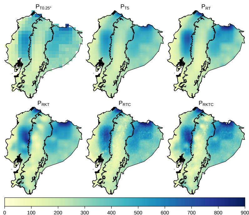
Figure 4. Monthly precipitation [mm] of April 2011 for the five products and the original TRMM data.
