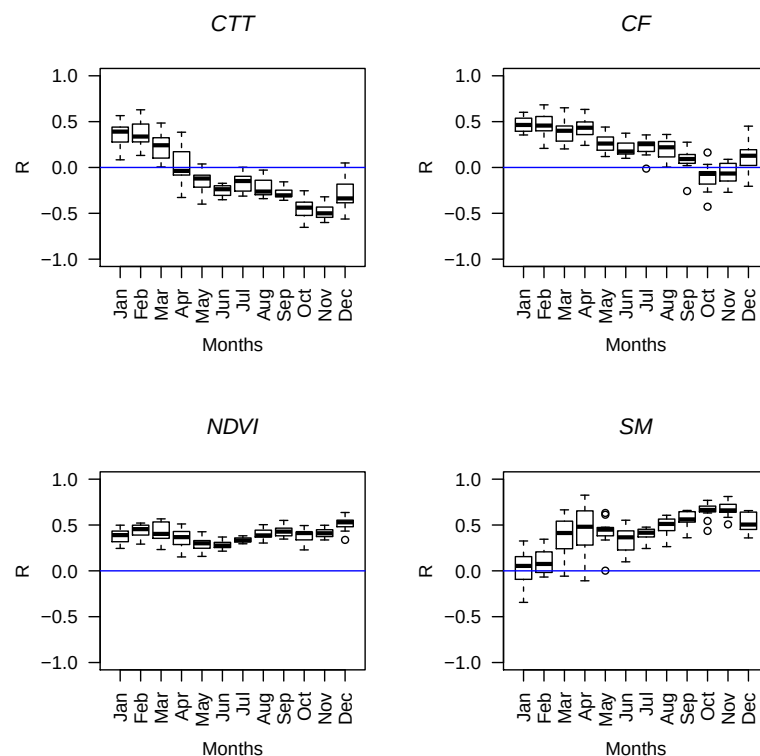
Figure 3. Correlation summary between each auxiliary variable and the observed precipitation data for the time period of study.
