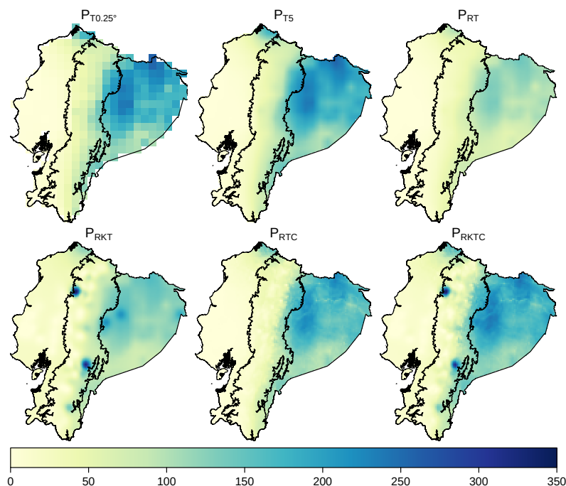
Figure 5. Monthly precipitation [mm] August 2011 for the five products and the original TRMM data.
