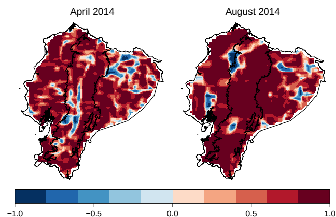
Figure 12. 5 \times 5 moving window correlation between the TRMM product and IMERG resampled to 5 km.
