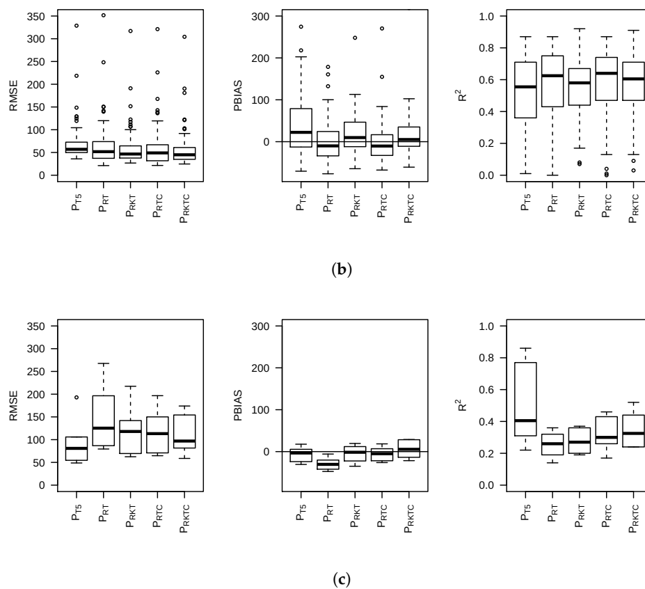
Figure 6. Summary of statistical values: (a) Coast region; (b) Andes region; (c) Amazon region.
