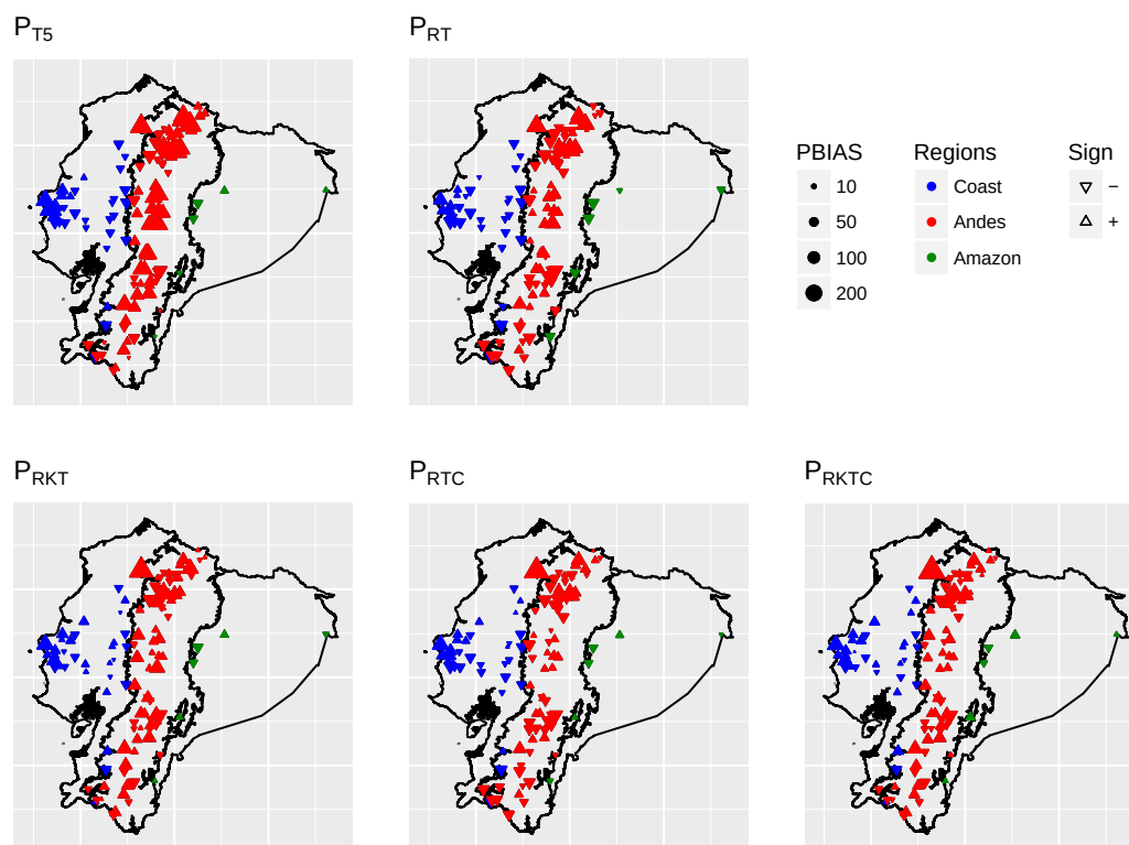
Figure 8. PBIAS of the five products over the station points.
