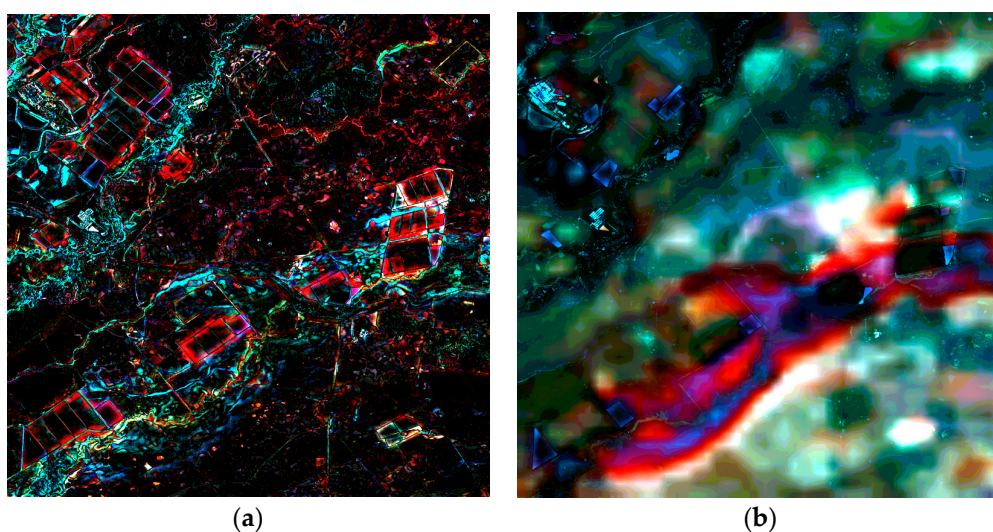
Figure 10. NIR-red-green composites of the squared error (with max values for bands NIR, red and green are 0.0025, 0.0011, and 0.0007) (a) and estimation variance (with max values for bands NIR, red and green are 0.0013, 0.0011 and 0.0008); (b) results for the third dataset.
