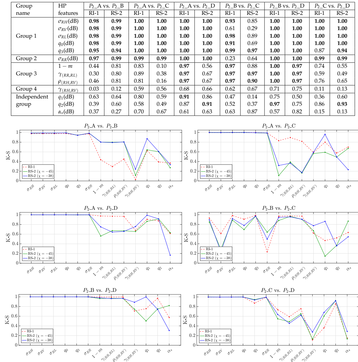
Figure 8. Top panel; a table containing the K-S values between all combinations of paired sea ice types in P_2 . The first column shows groups as described in Table 3. The values greater than 0.9 are in bold. Bottom panels; the corresponding values are shown in the plots, where the y-axis shows the K-S values calculated for each of the paired sea ice types (i.e., ROIs) (red for the RI-1 features and green (blue) for the RS-2 features with an ellipticity angle of \chi = -45^\circ ( -38^\circ )), while the x-axis shows the corresponding features. Note that only the K-S values for RI-1 features and the RS-2 features using an ellipticity angle of \chi = -45^\circ is shown in the table.
