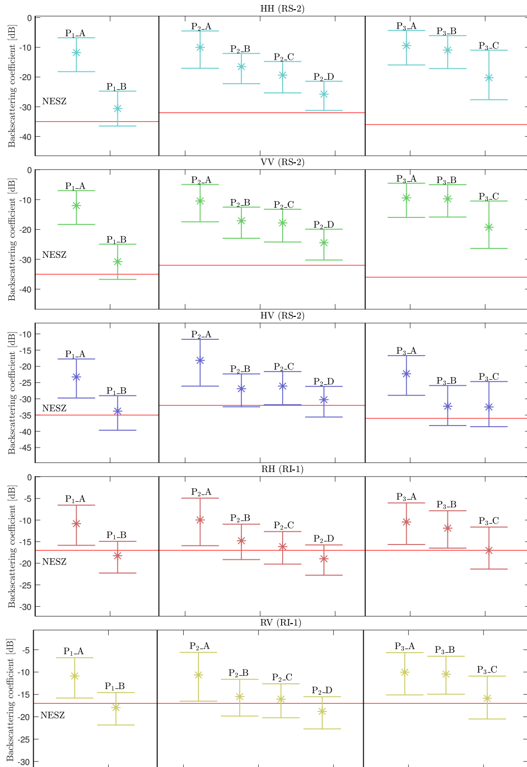
Figure 6. Signal-to-noise analysis of the backscattering intensity coefficients of the HH, VV, and HV for RS-2, and RH and RV for RI-1 for the investigated sea ice types. The 50th percentile is indicated by a star. The top and bottom horizontal continuous lines represent the 95th percentile and 5th percentile for the intensities, respectively. The red line represents NESZ. The y-axis represents the backscattering intensity coefficient, while the different sea ice types (i.e., ROIs) are aligned along the x-axis sorted by scene pair number.
